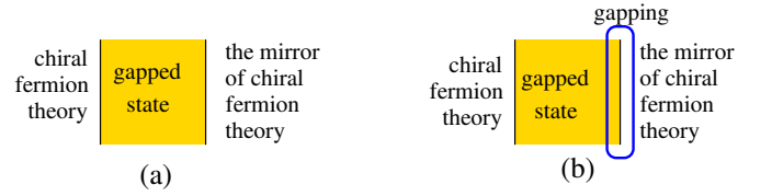
FIG. 4. (Color online) (a) Chiral fermions and mirror of chiral fermions can appear on the boundary of a 4+1d slab of gapped state. (b) Sometimes (such as the SO(10) case) the boundary mirror chiral fermions can be gapped by interaction, which leads to a solution of the chiral fermion problem.
