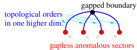
FIG. 1. (Color online) A general picture of a gapless quantum states, which is formed by decoupled anomalous gapless sectors restricted to the symmetric sub-Hilbert spaces (the red dots). The emergent symmetry and emergent anomalies are described by noninvertible gravitational anomalies ( i.e. the topological orders in one higher dimension). Thus, the anomalous sectors are the boundary of corresponding topological orders in one higher dimension.
