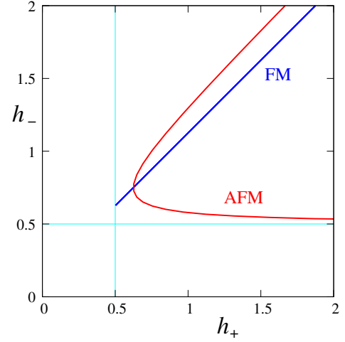
FIG. 2. The relations between the total scaling dimensions h_+ and h_- of the electron operators with Z_2^s quantum number \sigma^x = 1 and \sigma^x = -1 , respectively, for the ferromagnetic (FM) and anti-ferromagnetic (AFM) Ising transitions.
