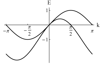
FIG. 3. The band structure of free fermions to construct chiral metallic phase. The two bands are for two flavors. Each band is double degenerate corresponding to two spin- \frac{1}{2} . Velocities v(k) at k = 0 are the same, and likewise v(\frac{\pi}{2}) = v(\pi) .
