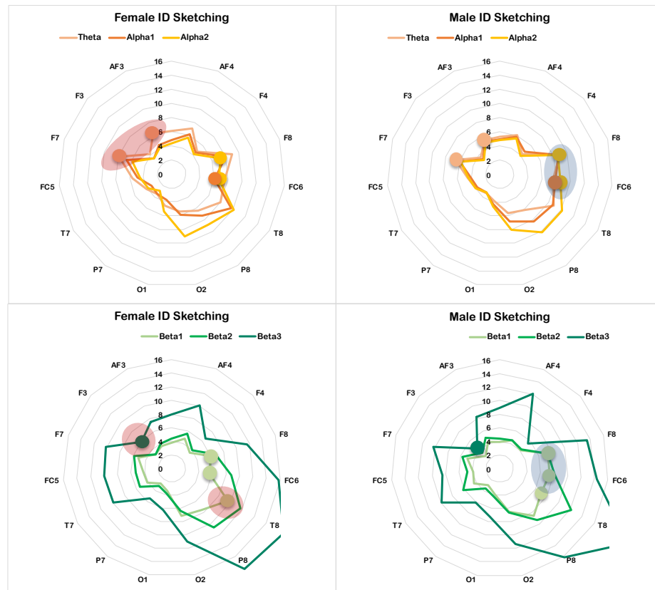
Figure 3. Transformed power ( Pow ) per channel for theta, alpha and beta frequency bands of the female and male industrial designers for the sketching stage. The solid circles indicate channels of moderate ( >.50 ) and large ( >.80 ) effect size. Shaded areas refer to higher frequency power in that group.
