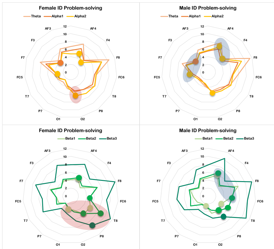
Figure 2. Transformed power (Pow) per channel for theta, alpha and beta frequency bands of the female and male industrial designers for the problem-solving stage. The solid circles indicate channels of moderate (>.50) and large (>.80) effect size. Shaded areas refer to higher frequency power in that group.
