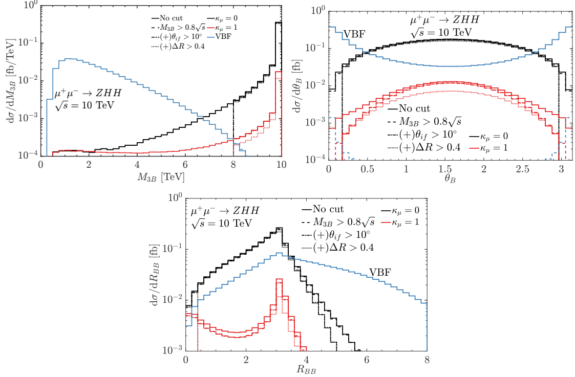
Figure 10. The kinematic distributions for \theta_B , R_{BB} , and M_{3B} as in figure 9, but for ZHH production at a \sqrt{s} = 10 TeV \mu^+\mu^- collider.
