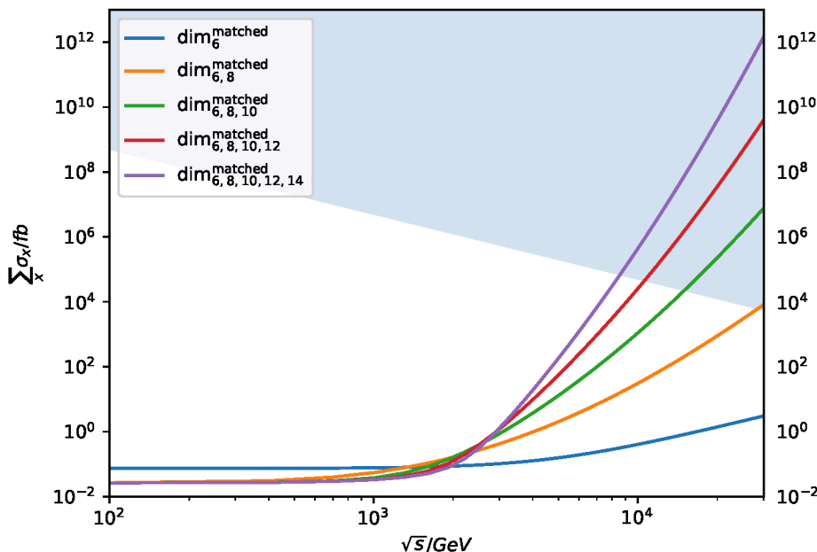
Figure 3. Inclusive inelastic cross section \mu^+\mu^- \rightarrow X for multiple Goldstone and Higgs-boson production in the GBET approximation. We show the result for the sequence of SMEFT scenarios defined by the conditions (2.25), truncated at dimension d = 6, 8, 10, 12, 14 , respectively. The maximal multiplicity of the final state is n = 3, 5, 7, 9, 11 , respectively. The shaded area indicates the region that is excluded by the universal unitarity bound for the inclusive cross section (2.33).
