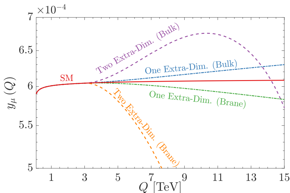
Figure 1. LO RGE running of the muon Yukawa y_\mu coupling as a function of the energy scale Q , in the SM (red solid). In the extra-dimensional scenarios (with inverse radius 1/R = 3 TeV), we consider 1) Bulk: all fields propagating in the bulk, and 2) Brane: all matter fields localized to the brane.
