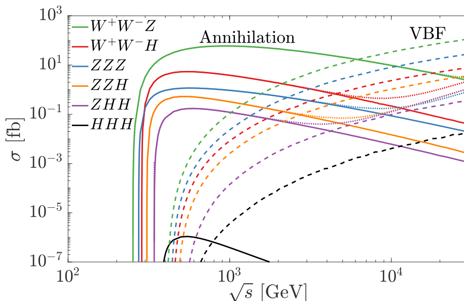
Figure 5. Similar to figure 4, the cross sections of three-boson production at a \mu^+\mu^- collider as a function of the c.m. energy \sqrt{s} .
