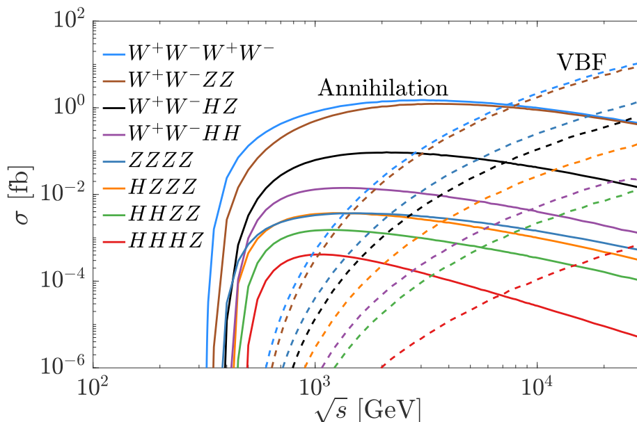
Figure 6. Similar to figure 4, the cross sections of four-boson production at a \mu^+\mu^- collider as a function of the c.m. energy \sqrt{s} , for SM \kappa_\mu = 1 only.
