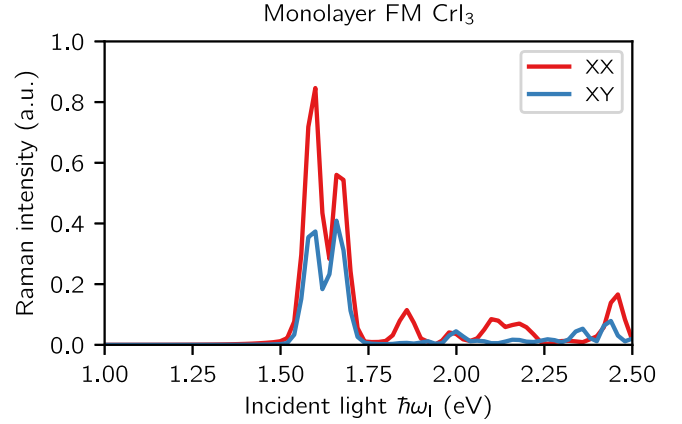
FIG. 3. The calculated Raman intensity of A_g mode in monolayer ferromagnetic \text{CrI}_3 . The photon energy on the horizontal axis is shifted to reproduce the GW-BSE calculated optical band-gap onset. The vertical scale here can not be compared with the bulk calculation from Fig. 1 due to the reduced dimensionality of the monolayer as compared to bulk.
