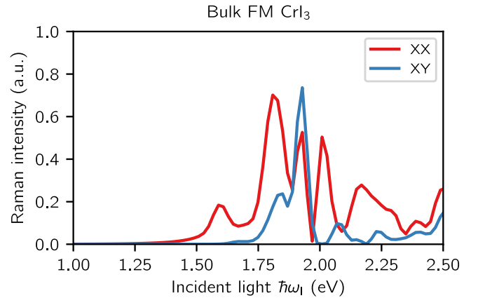
FIG. 1. The calculated Raman intensity of A_g mode in bulk ferromagnetic \text{CrI}_3 . The photon energy on the horizontal axis is shifted to reproduce the GW-BSE calculated optical band-gap onset.
