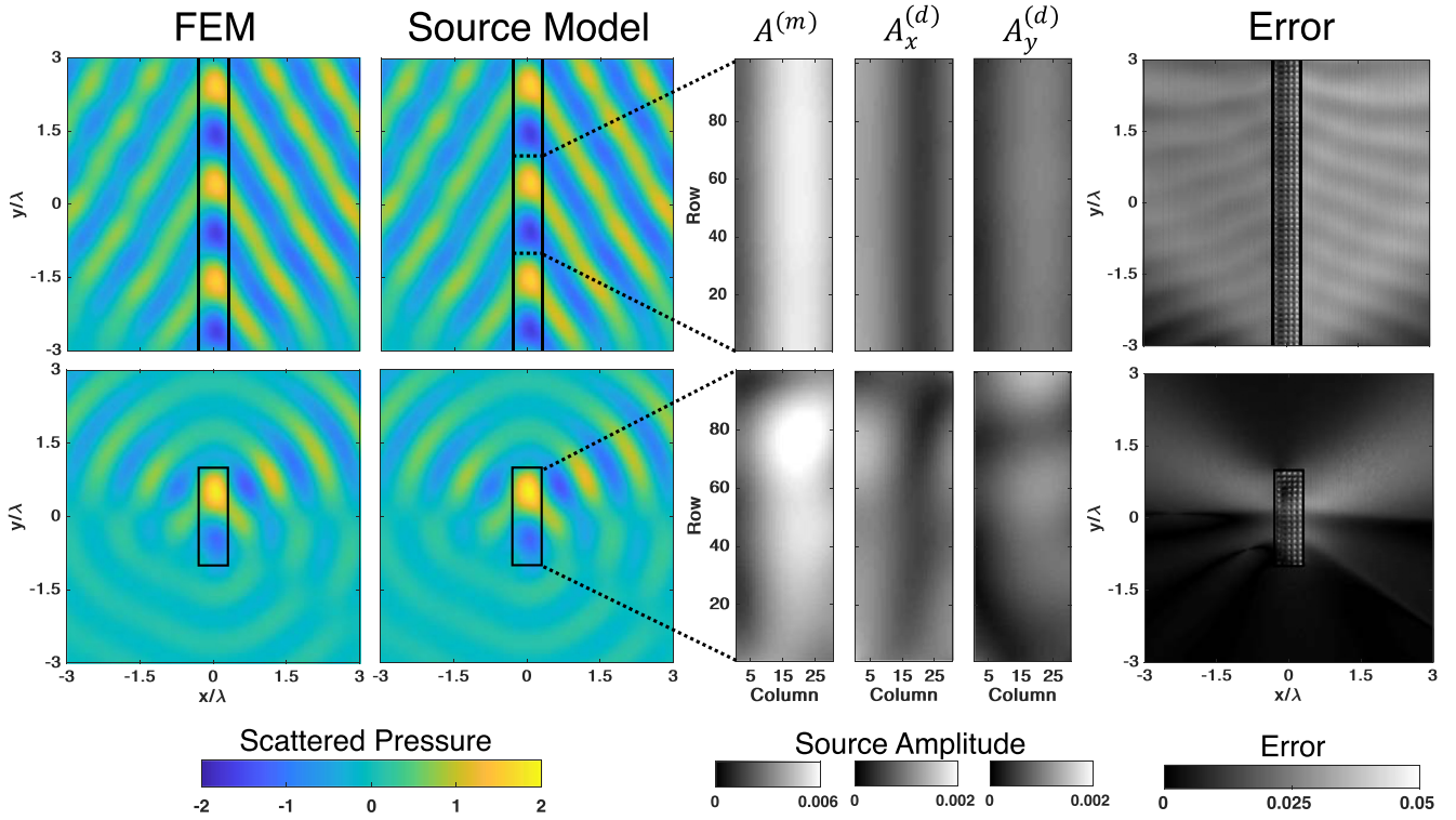
FIG. 2. Scattering from a plane wave obliquely incident on acoustically short and tall slabs (outlined in black) of \kappa_{\text{eff}} = 3 and \rho_{\text{eff}} = 2 is compared between an FEM and source model simulation. The amplitudes of the sources in the cell lattice are shown for slab sections of equal dimension. The error of the source model scattered field amplitude is plotted relative to the maximum pressure in the simulated region.
