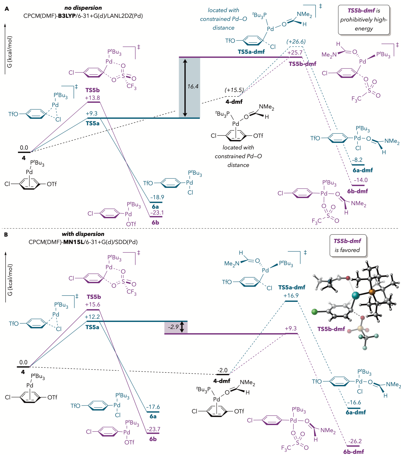
Figure 2. Effect of dispersion on the stability of DMF-coordinated oxidative addition transition structures. Free energy values are corrected for concentration (DMF: Pd = 765:1) and are reported after applying Cramer and Truhlar's 29 and Head-Gordon's 30 quasi-harmonic approximations to vibrational entropy and enthalpy, respectively. 31,32
