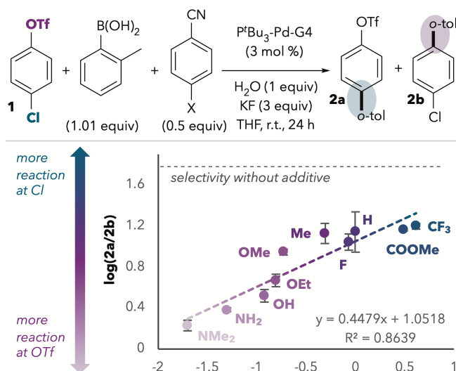
Figure 1. Hammett-type plot shows a correlation between benzonitrile donor ability and increasing reaction at triflate. Each data point represents the average of three trials, and the error bars represent standard deviation.
