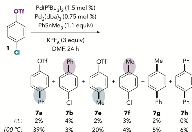
Scheme 3. Base-Free Stille Coupling of 1 Catalyzed by Pd/P t Bu 3 . GC yields calibrated against dodecane as an internal standard. Results are the average of two trials. Leftover 1 : 83% at r.t., 4% at 100 °C.
