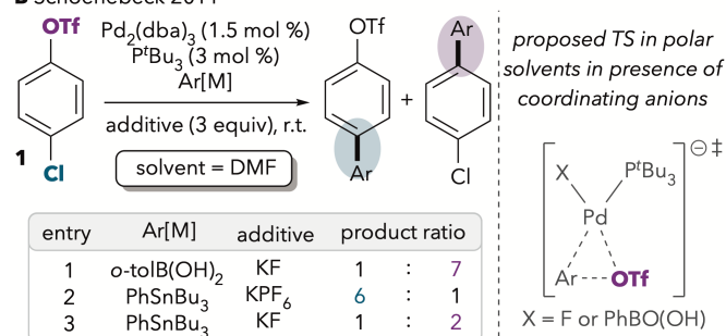
Scheme 1. Seminal Reports on the Effects of Ligands and Solvents on the Selectivity of Cross-Coupling of a Chloroaryl Triflate 5,7,9
