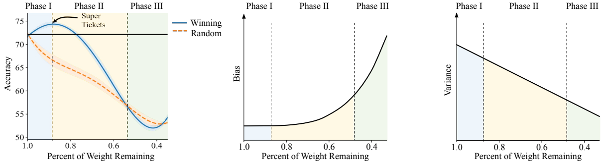
Figure 1: Illustrations of the phase transition phenomenon. Left: Generalization performance of the fine-tuned subnetworks (the same as Figure 4 in Section 5). Middle and Right: An interpretation of bias-variance trade-off.
