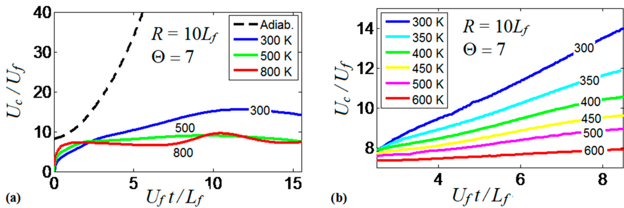
Figure 9. The scaled flame velocity at a channel centerline U_c/U_f versus the scaled time U_f t/L_f for a flame with a thermal expansion ratio \Theta = 7 propagating in a channel of half-width R = 10L_f with nonslip walls: (a) adiabatic (dashed) and isothermal (solid) walls with T_w = 300 K, 500 K and 800 K; (b) isothermal walls with T_w in the range from 300 K till 600 K.
