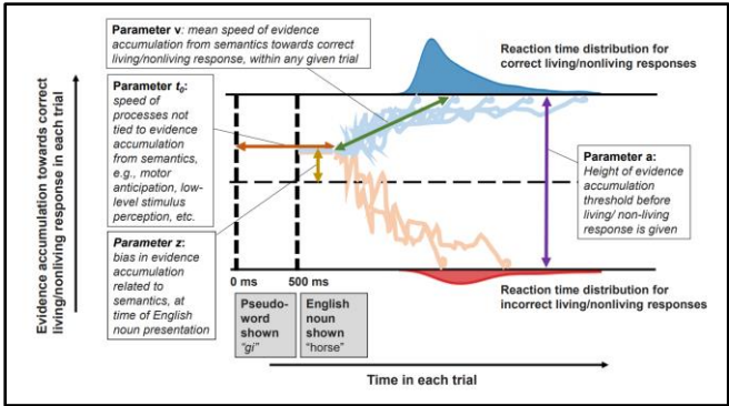
Figure 1: Visualization of drift-diffusion model in the context of our experiment paradigm. Not pictured: parameters capturing standard deviation of v , t_0 , and z Visualization inspired by Fig. 1 in Vinding et al. (2018)
