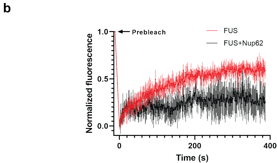
Supplemental Figure 8: FRAP measurements of recombinant FUS/Nup proteins. (a) Time lapse fluorescence images of FRAP experiment. MBP-FUS/Nup62 assemblies (top panel) and MBP-FUS droplets formed without addition of Nup62 (bottom panel) were photobleached and the fluorescence recovery was monitored. Image taken before bleaching (pre-bleach), immediately after bleaching (post-bleach: 0s) and endpoint (post-bleach: 386s) are shown. Yellow circle outlines the bleach region. Supplemental Video 1 and 2 correspond to these FRAP measurements. Results are representative of n=5 and n=6 FUS and FUS/Nup62 assemblies respectively. Scalebar = 5\mu\text{m} . (b) Fluorescence recovery curves of FRAP experiment on FUS droplets (red curve, n=6 droplets) and FUS/Nup62 aggregates (black curve, n=5 regions). Error bars represent standard deviation. The custom code for this analysis has been provided as supplemental material (code_frap_invitro.py).
