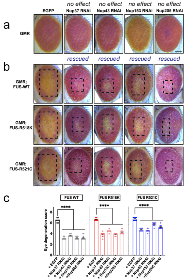
Supplemental Figure 15. RNAi-mediated knockdown of Nup37, Nup43, Nup153 and Nup205 results ameliorates FUS-induced eye degeneration. (a) Representative images of eye phenotypes of flies expressing RNAi for Nup37, Nup43, Nup153, and Nup205 indicates no external eye degeneration. (b) Representative images of fly eyes showing that external eye degeneration, indicated by areas of depigmentation and ommatidial fusion, caused by expression of FUS WT and mutants (R518K and R521C) are suppressed by Nup27, Nup43, Nup153 and Nup205 RNAi. Black dashed boxes highlight areas of marked eye degeneration; the size of the box corresponds to the area of degeneration. Scale bar= 100µm. (c) Quantification of eye degeneration (from b) indicates statistically significant difference in eye phenotypes upon modulation of nucleoporins in FUS WT, FUS R518K and FUS R521C backgrounds (FUS-WT+EGFP, n=48; FUS-R518K+EGFP, n=48; FUS-R521C+EGFP, n=48; FUS-WT+Nup37/Nup43/Nup153/Nup205 RNAi, n=20; FUS-R518K+Nup37/Nup43/Nup153/Nup205 RNAi, n=20; FUS-R521C+Nup37/Nup43/Nup153/Nup205 RNAi, n=20). Each point represents one adult fly, Kruskal-Wallis test with Dunn's multiple comparisons test was used for analysis. ****p-
