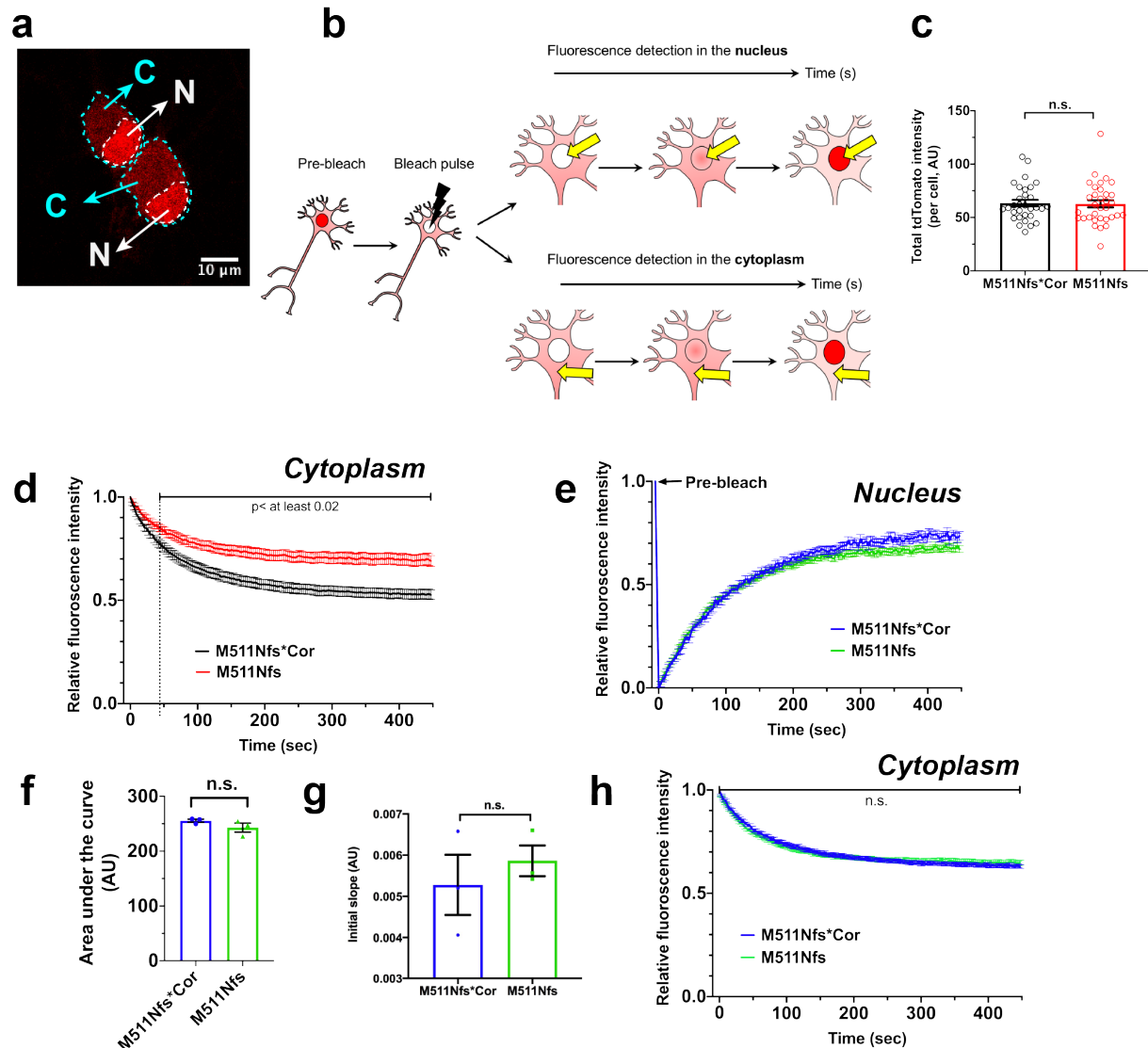
Supplemental Figure 5. Additional live-cell fluorescence analysis of the NLS-tdTomato-NES shuttling reporter in ALS-FUS human neurons. (a) Representative image of the transduced NLS-tdTomato-NES shuttling reporter (red) in human neurons. The fluorescence signal for this reporter construct is diffuse and predominately localized to the nucleus. Scale bar= 10 \mu m. N=nucleus, C=cytoplasm. (b) Illustration for FRAP analysis. Top panel: Fluorescence detection in the nucleus monitors the import of unbleached tdTomato (red) from the cytoplasm. Nuclear red fluorescence increases over time as a function of tdTomato (red) import. Since there are fewer fluorescent molecules in the cytoplasm to begin with, the fluorescence never fully recovers in the nucleus on the time-scale of this experiment. Bottom panel: Fluorescence detection in the cytoplasm measures bleached tdTomato (non-fluorescent or “white”) exported from the nucleus. The red fluorescence in the cytoplasm decreases as the red signal becomes diluted with bleached molecules exported from the nucleus. Yellow arrows indicate the area of the cell where the fluorescence is detected as a function of time. (c) The total reporter expression level/ transduction efficiency was similar in FUS M511Nfs and control. M511Nfs*Cor: n=29 cells; M511Nfs: n=36 cells, examined from n=3 independent
