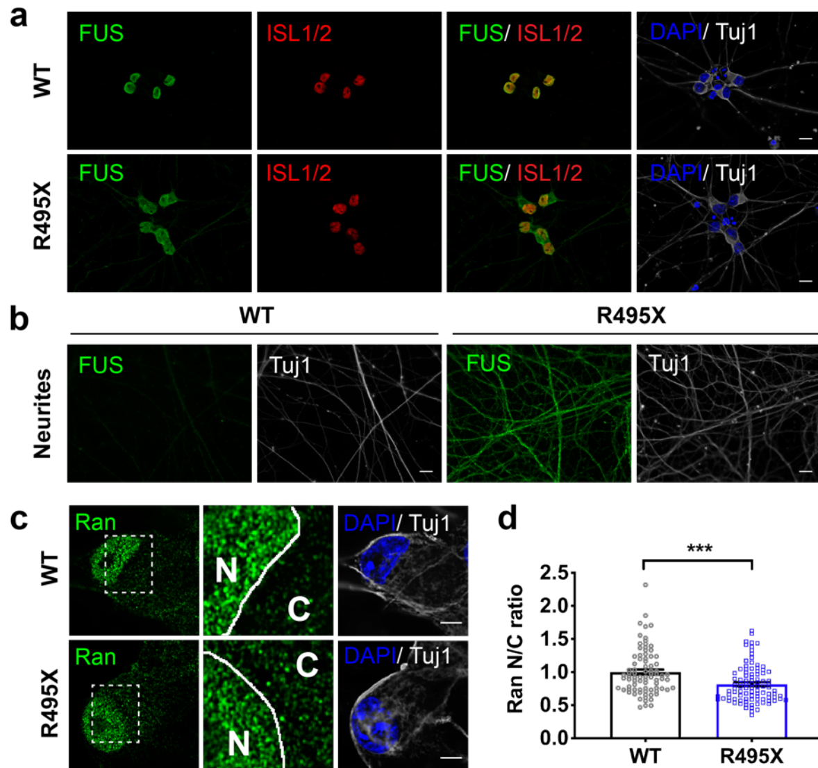
Supplemental Figure 3. Differentiation and assessment of the Ran gradient in isogenic FUS R495X iPSC lines. (a) Immunofluorescence image of FUS in iPSC-derived neurons. ISL1/2 (red), DAPI (blue), Tuj1 (grey). (b) FUS staining in the neurites of iPSC-derived neurons. Scale bar= 10 \mu m. (a,b) Images are representative of n=1 experiments. (c) Immunofluorescence image of Ran (green), DAPI (blue), Tuj1 (grey), representative of n=3 experiments. The Ran N/C ratio of the chosen representative neurons: WT (1.25); R495X (0.87). Abbreviation within the zoom insets: N (nucleus), C (cytoplasm). Neurons at DIV 56 (8 weeks) were used for this analysis. Scale bar= 10 \mu m. (d) Quantification of the Ran N/C ratio. Ran N/C is significantly lower in R495X versus WT neurons (WT, n=82; R495X, n=95 cells; from n=3 independent biological replicates). Unpaired two-tailed t-test, ***p=0.0001, t=3.935, df=175. Error bars represent s.e.m. Data distribution was assumed to be normal but this was not formally tested.
