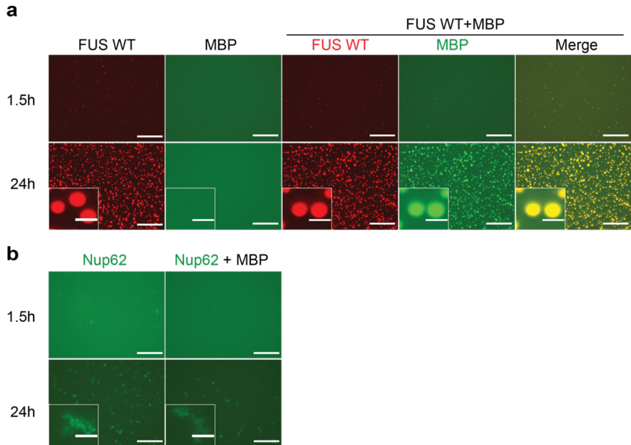
Supplemental Figure 11. MBP does not alter FUS or Nup62 phase separation. (a) Fluorescence images showing phase separation of 1.5 \mu M MBP-FUS WT (red) doped with 2.5% Alexa555-labelled MBP-FUS WT. MBP-FUS droplet formation is not altered by co-incubation with 1.5 \mu M MBP-MBP (green; doped with 1% Alexa488 labelled MBP), although MBP is detected within FUS droplets. (b) Fluorescence images showing amorphous assemblies of 1.5 \mu M MBP-Nup62 (green) doped with 2.7% Alexa488 labelled MBP-Nup62. Formation of MBP-Nup62 amorphous assemblies is not enhanced upon co-incubation with 1.5 \mu M MBP (unlabeled). Images were taken at the indicated timepoints after initiation of phase separation by 3.6% PEG. Results are representative of n=4 (for panel A) and n=2 (for panel B) independent experiments. Scale bar= 50 \mu m (inset = 5 \mu m).
