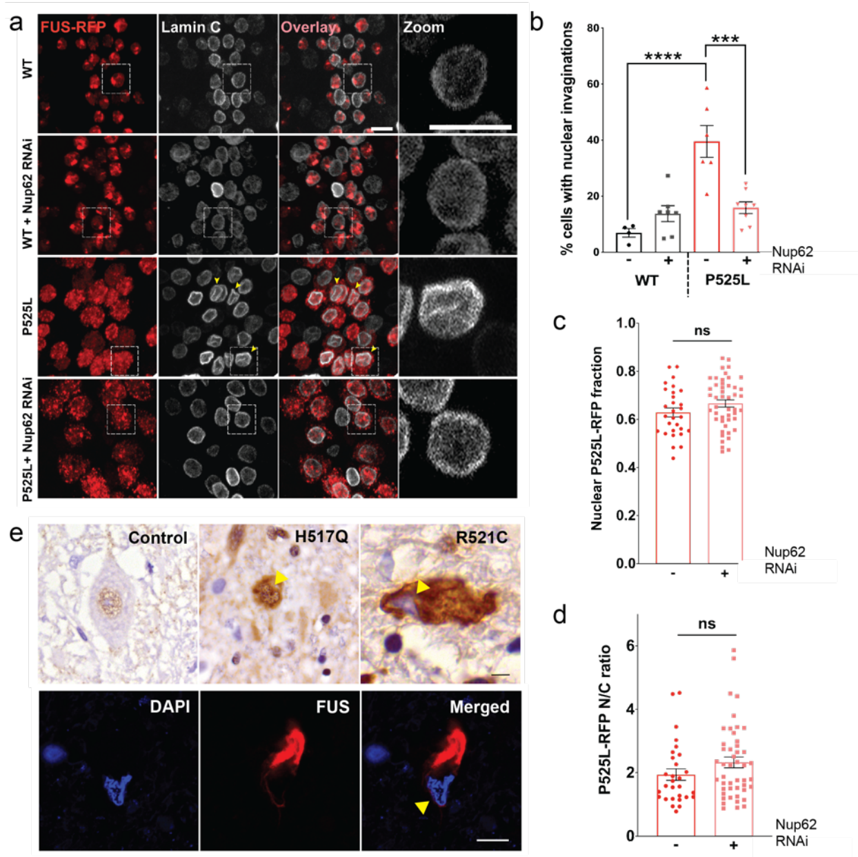
Figure 6. Nuclear abnormalities associated with ALS-linked FUS are rescued by knock-down of Nup62 in vivo (a) Immunofluorescence imaging of larval ventral nerve chord in Drosophila expressing FUS WT-RFP (red, top) and ALS mutant FUS P525L-RFP (red, bottom), with and without Nup62 knockdown. Lamin C (grey) staining was used to mark the nuclear membrane. Nuclear membrane invaginations, which appear as wrinkled membranes, were observed in P525L-expressing neurons (denoted by yellow arrowheads). Zoom images show normal nuclear membrane morphologies for all conditions except P525L. Scale bar= 10µm. (b) Quantification of percentage of neurons that have nuclear membrane defects in all four groups (Each point in the bar graph
