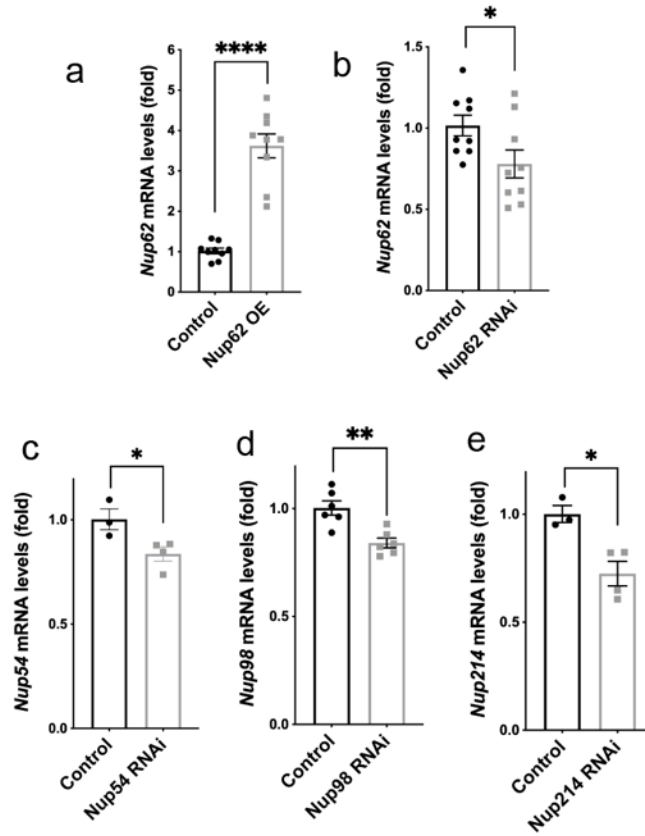
Supplemental Figure 14. Nups mRNA levels in flies measured in fly heads after overexpression or knock-down. Quantification plots of fold-change differences in mRNA levels shows (a) statistically significant overexpression (OE) of transgenic Nup62 (fold change = 3.6; Control, n=9; Nup62 OE, n=9), and statistically significant RNAi-mediated knockdown of (b) Nup62 (fold change = 0.77; Control, n=9; Nup62 RNAi, n=9), (c) Nup54 (fold change = 0.85; Control, n=3; Nup54 RNAi, n=4), (d) Nup98 (fold change = 0.84; Control, n=6; Nup98 RNAi, n=6) and (e) Nup214 (fold change = 0.72; Control, n=4; Nup214 RNAi, n=4) compared to w1118 Control. (a-e) Each point represents a technical replicate. Unpaired Two-tailed Student's t-test was used for analysis. (For [a]: t=8.542 , df = 16 ; for [b]: t=2.211 , df = 16 ; for [c]: t=2.85 , df = 5 ; for [d]: t=4.05 , df = 10 ; for [e]: t=3.689 , df = 5 ) ****p-value<0.0001; Control vs Nup62 RNAi p-value=0.0420; Control vs Nup54 RNAi p-value=0.0358; Control vs Nup98 RNAi p-value=0.0023; Control vs Nup214 RNAi p-value=0.0142. Data distribution was assumed to be normal but this was not formally tested. Error bars indicate s.e.m.
