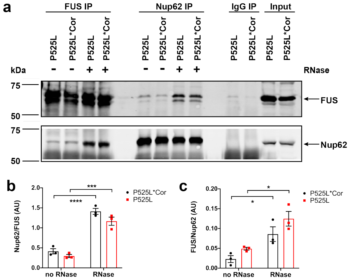
Figure 3. Wild-type and mutant FUS interact with Nup62 in iPSCs. (a) Left: FUS IP. Nup62 was pulled down with wild-type (P525L*Cor) and mutant (P525L) FUS. Middle: Nup62 IP. Both wild-type and mutant FUS were pulled down with Nup62. In both IPs, interactions of FUS and Nup62 were retained and significantly enhanced upon RNase treatment, suggesting the interactions were not mediated through RNA. Right: IgG and input controls for IP. Source data are provided as a Source Data file. (b) Quantification for FUS IP. Densitometry analysis of FUS and Nup62 signals in the Western blot shown in (a). Two-way ANOVA with Tukey's multiple comparisons test. P525L*Cor: **** p < 0.0001 ; P525L: *** p = 0.0002 . F(1, 8) = 0.7543 . (c) Quantification for Nup62 IP, as described for (b). Two-way ANOVA with Tukey's multiple comparisons test. P525L*Cor: * p = 0.0497 ; P525L: * p = 0.0204 . F(1, 8) = 0.2072 . Only significant comparisons were denoted. (b,c) Each point in the bar graph represents a biological replicate ( n = 3 ). Error bars represent s.e.m. Data distribution was assumed to be normal but this was not formally tested.
