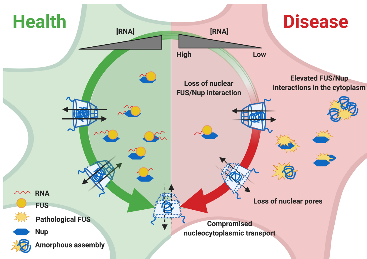
Supplemental Figure 19. Proposed model for how aberrant mutant FUS/Nup62 interactions contribute to nucleocytoplasmic transport decline. The efficiency of nucleocytoplasmic transport declines with age (left) and may be accelerated in neurodegenerative disorders (right). Mutations in the nuclear localization sequence of FUS cause the protein to mislocalize and accumulate in the cytoplasm (right). Our data uncovered direct interactions between FUS and nucleoporins, including Nup62. In control neurons, FUS/Nup interactions are enriched within the nucleus (left). Conversely, in ALS-FUS neurons (right), FUS/Nup interactions and Nup/Nup interactions are enriched within the cytoplasm, where relatively low levels of RNA could favor aberrant FUS/Nup interactions. Consistent with this model, recombinant FUS and Nup62 proteins alter the phase separation properties of each other, where FUS transitions from a liquid droplet into a less dynamic amorphous assembly under conditions of low RNA concentration. Over time, the accumulation and stabilization of cytoplasmic mutant FUS/Nup complexes in neurons is expected to reduce Nup occupancy at the nuclear membrane, thereby reducing NCT capacity and cell health. Decreasing Nup expression rescues toxic FUS phenotypes in flies, including abnormal nuclear membrane morphology in mutant FUS neurons. Collectively, our results indicate the mislocalization of mutant FUS to the cytoplasm within neurons, rather than a physicochemical property of the FUS protein itself, facilitates aberrant interaction with Nups.
