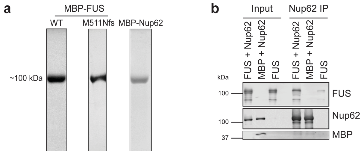
Supplemental Figure 7. Characterization of recombinant proteins and binding of FUS with Nup62. (a) Coomassie blue staining of purified MBP-FUS WT, MBP-FUS M511Nfs and MBP-Nup62. Results are representative of n=3 (MBP-FUS WT), n=1 (MBP-FUS M511Nfs) and n=3 (MBP-Nup62) independent purifications. Source data are provided as a Source Data file. (b) Recombinant MBP-FUS binds to MBP-Nup62: Western blot of co-IP binding assay showing that MBP-FUS co-elutes when MBP-Nup62 is pulled down with an anti-Nup62 antibody from a mixture containing MBP-FUS and MBP-Nup62. This interaction is not mediated by the MBP tag as MBP protein in the absence of MBP-FUS fails to co-elute with MBP-Nup62. Results are representative of n=2 independent experiments. Source data are provided as a Source Data file. These experiments serve to validate the following antibodies: rabbit anti-Nup62 antibody (Bethyl Laboratories, A304-942A), which was used to charge the beads and to probe for nup62 in the Western blot; mouse anti-FUS (Santa Cruz, SC-373698), which was used to probe for FUS in the Western blot; and mouse anti-maltose binding protein (Cell Signalling Technology, 2396), which was used to probe for MBP in the Western blot.
