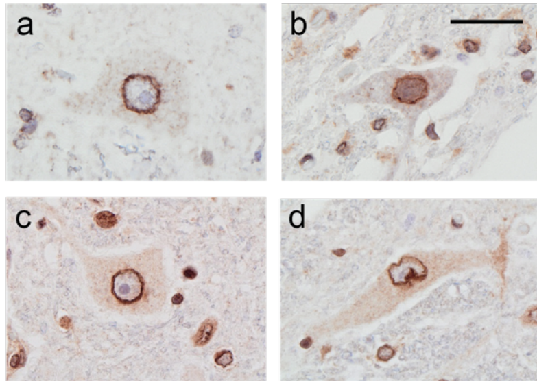
Supplemental Figure 17. Nup62 immunohistochemistry of human post-mortem spinal cord tissue. In the ALS-FUS R521G case (a and b) some lower motor neurons had normal nuclear morphology and strong Nup62 staining of the nuclear membrane (a) but many showed either abnormal morphology or Nup62 staining that was not confined to the nuclear membrane (b). In the control sections (c and d), most of the neurons had normal appearing Nup62 signal (c) but there were also some with abnormal morphology (d). ( a-d ) Images are representative of n=1 staining experiments. Scale bar = 50 \mu m.
