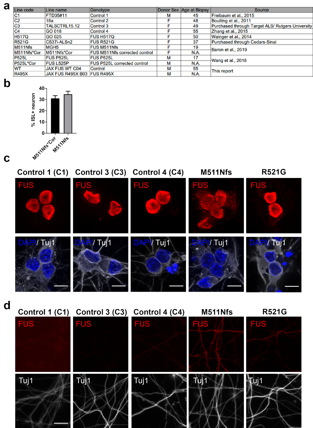
Supplemental Figure 1. iPSC lines and immunofluorescence images of FUS localization. (a) Table of iPSC lines used in this report 10,23,28,65-67 . (b) Percentages of motor neurons yield from n=3 independent differentiations of FUS M511Nfs isogenic lines. Error bars represent s.e.m. (c) Immunofluorescence images of FUS in iPSC-derived
