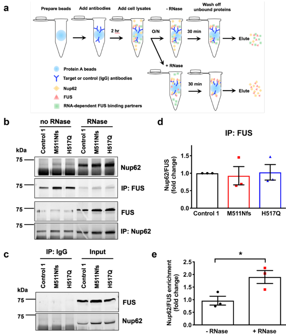
Supplemental Figure 6. Additional analyses of FUS/Nup62 binding in iPSCs. (a) Schematic co-immunoprecipitation (IP) experimental design. (b) Top 2 blots: FUS IP. Nup62 was pulled down with control and mutant (M511Nfs and H517Q) FUS. Bottom 2 blots: Nup62 IP. Both wild-type and mutant FUS were pulled down with Nup62. In both IPs, interactions of FUS and Nup62 were retained and significantly enhanced upon RNase treatment, suggesting the interactions were not mediated through RNA. Source data are provided as a Source Data file. (c) IgG and input controls for IP. Source data are provided as a Source Data file. (d) Quantification for FUS IP. Densitometry analysis of FUS and Nup62 signals in the Western blot shown in (b). One-way ANOVA with Tukey's multiple comparisons test. Control v.s. M511Nfs: p=0.8047 . Control v.s. H517Q: p=0.9316 . F(2, 6)=0.06531 . (e) Quantification for FUS IP with and without RNase treatment. Unpaired two-tailed t-test. *p=0.0391 . t=3.021 , df=4 . Each point in the bar graph represents a biological replicate. Error bars represent s.e.m. (d,e) Data distribution was assumed to be normal but this was not formally tested.
