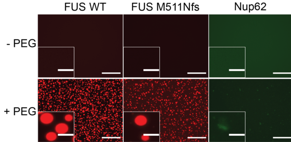
Supplemental Figure 10. FUS and Nup62 assemblies form only in the presence of PEG. Fluorescence images showing absence of FUS or Nup62 assemblies when PEG is not added (top). FUS and Nup62 assemblies are formed only upon addition of 3.6% PEG (bottom). MBP-FUS WT and -M511Nfs (1.5 \mu M) are doped with 2.5% Alexa555-labelled FUS WT or -M511Nfs and MBP-Nup62 (1.5 \mu M) is doped with 2.7% Alexa488 labelled MBP-Nup62. Images were taken 24h after addition of PEG. Results are representative of n=4 independent experiments. Scale bar= 50 \mu m (inset = 5 \mu m).
