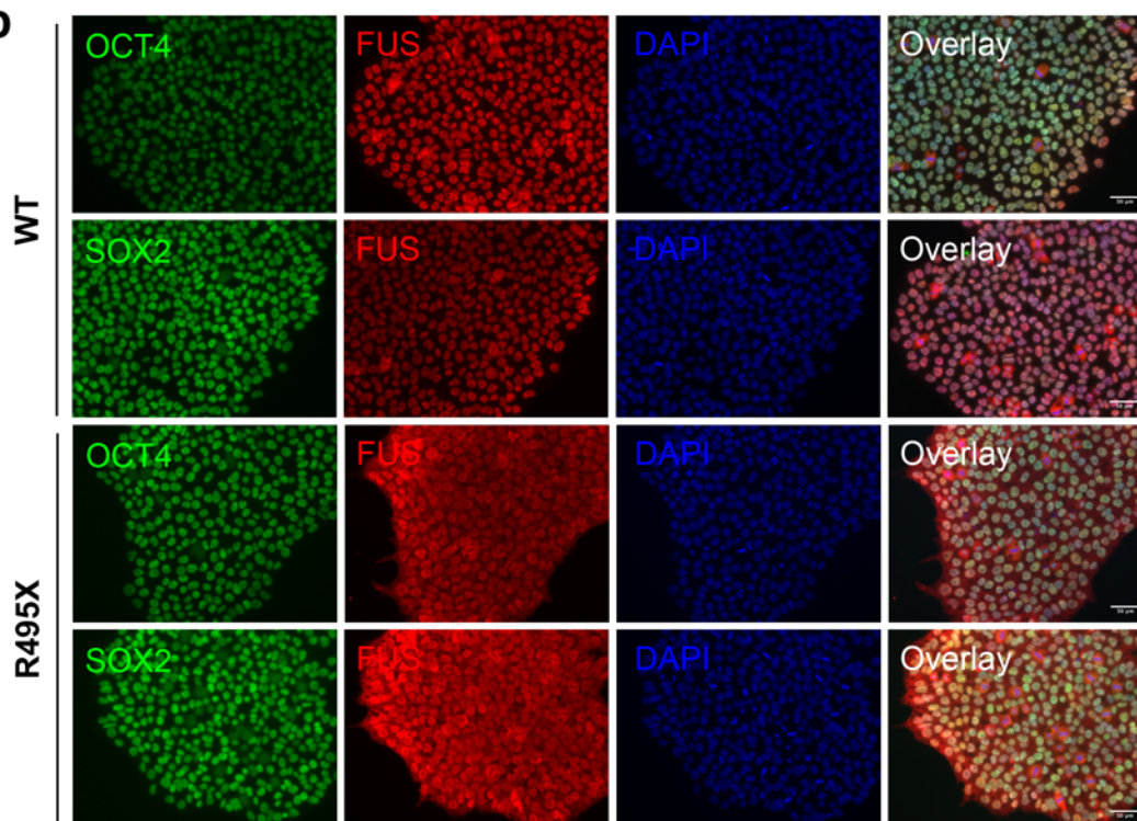
Supplemental Figure 2. Generation of FUS R495X isogenic induced pluripotent stem cells. (a) Results of Sanger sequencing after gene-editing to introduce the FUS R495X mutation. (b) Immunofluorescence image of pluripotency markers OCT4 and SOX2 (green) and FUS (red) in iPSCs, representative of n=1 experiments. DAPI (blue). Scale bar= 50 \mu m.
