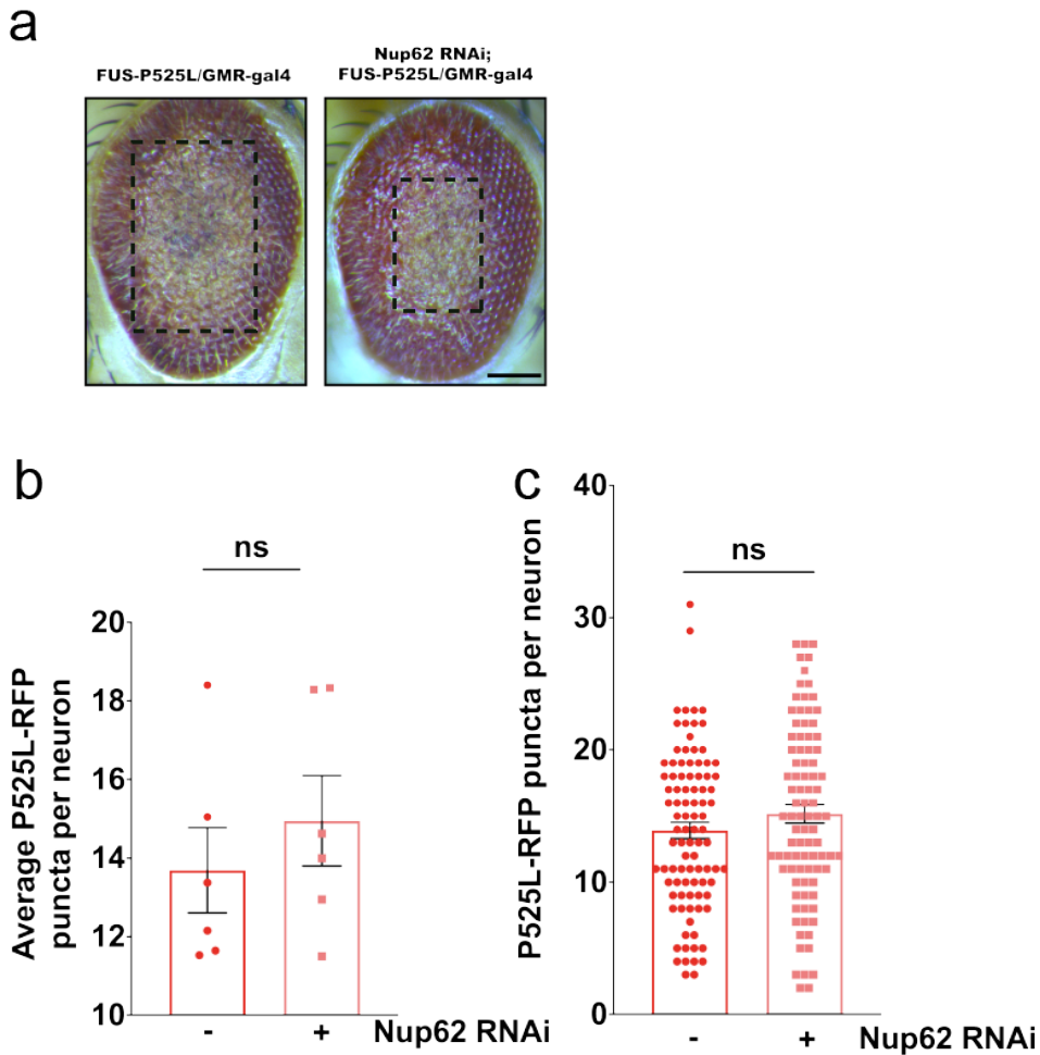
Supplemental Figure 16. Phenotypes in flies due to expression of FUS P525L. (a) Representative images of fly eyes showing that external eye degeneration, indicated by areas of depigmentation and ommatidial fusion, caused by expression of FUS P525L mutant alone (left) and suppressed eye degeneration upon co-expression with Nup62 RNAi (right). Black dashed boxes highlight areas of marked eye degeneration; the size of the box corresponds to the area of degeneration. Scale bar= 100 \mu m (b-c) Quantification of P525L-RFP puncta in larval ventral nerve cord neurons shows no significant differences in (b) average number of puncta per neuron (p-value=0.4447) or (c) the number of puncta in each individual neuron pooled across all larva with or without Nup62 knockdown (p-value=0.1768) (n = 6 larvae per genotype; P525L-RFP n = 94 neurons; P525L+Nup62 RNAi n = 90 neurons). Each point represents data from one larva in (b), and one neuron in (c). (b) Data distribution was assumed to be normal but this was not formally tested. (c) Normality was tested using the Kolmogorov-Smirnov test on Prism Graphpad and the data was determined to have normal distribution. (b,c) Two-tailed Student's T-test used for analysis (For [b]: t=0.7956 , df = 10 ; for [c]: t=1.356 , df = 182 ). ns = not significant. Error bars indicate s.e.m.
