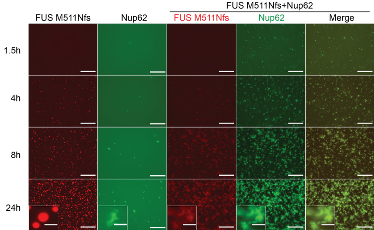
Supplemental Figure 9. Nup62 alters FUS M511Nfs phase separation in a similar manner to FUS WT. Fluorescence images showing phase separation of 1.5 \mu M MBP-FUS M511Nfs (red) doped with 2.5% Alexa555-labelled MBP-FUS M511Nfs. MBP-FUS droplet formation is altered by co-incubation with 1.5 \mu M MBP-Nup62 (green; doped with 2.7% Alexa488 labelled MBP-Nup62). Images were taken at the indicated timepoints after initiation of phase separation by 3.6% PEG. Results are representative of n=4 independent experiments. Scale bar= 50 \mu m (inset = 5 \mu m).
