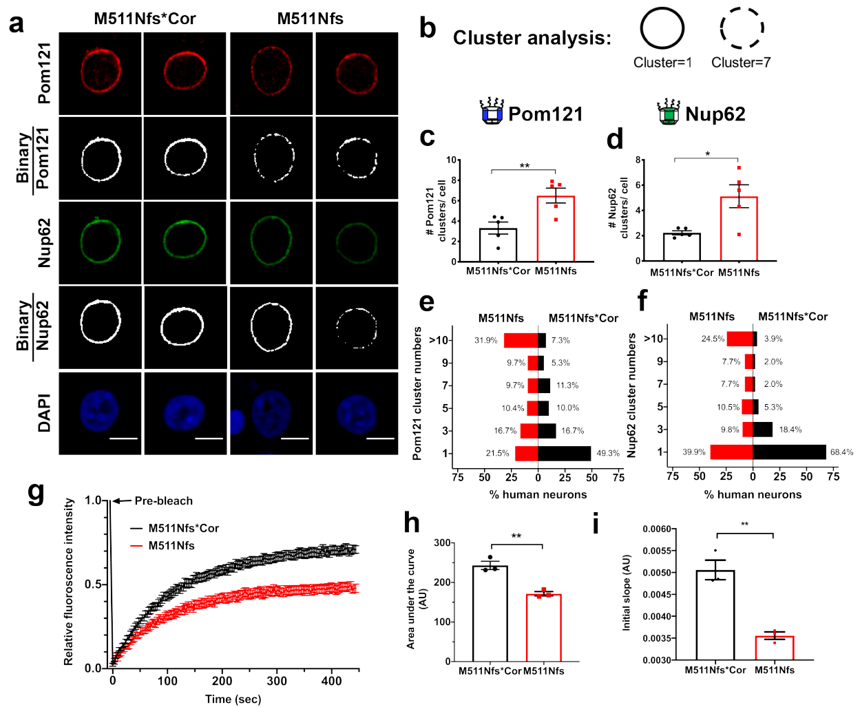
Figure 2. Diminished nuclear pore signal and nucleocytoplasmic transport in ALS-FUS human neurons. (a) Immunofluorescence images of Pom121 (red) and Nup62 (green), representative of n=5 experiments, reveals weaker signals in FUS M511Nfs nuclei compared to nuclei from the isogenic control neurons. Binary images (white) derived from the fluorescence images are shown. DAPI (blue). Scale bar = 5 \mu m. (b) An illustration for the cluster analysis used to quantify the continuity of Pom121 and Nup62 staining around the perimeter of the nucleus. (c-f) Results of the cluster analysis for Pom121 (scaffold Nup; c, e) and Nup62 (central channel Nup; d, f) for n=152 M511Nfs*Cor and n=144 M511Nfs nuclei that were analyzed across five independent differentiations (each differentiation represents an experiment) from neurons at DIV 36-45. (c, d): significantly higher cluster numbers in FUS M511Nfs versus M511Nfs*Cor nuclei through analysis of Pom121 (Unpaired two-tailed t-test, **p=0.0095 , t=3.391 , df=8 ) and Nup62 (Unpaired two-tailed t-test, p=0.0137 , t=3.144 , df=8 ; error bars represent s.e.m.). (e, f): results of the cluster analysis presented in a population pyramid format show the cluster number for every neuron analyzed. Each point in a bar graph represents the average across all cells in that experiment, normalized to M511Nfs*Cor. (g-i) Results of the FRAP experiment with the NLS-tdTomato-NES shuttling reporter in FUS M511Nfs*Cor neurons (black; n=29 cells) and M511Nfs neurons (red; n=36 cells) across
