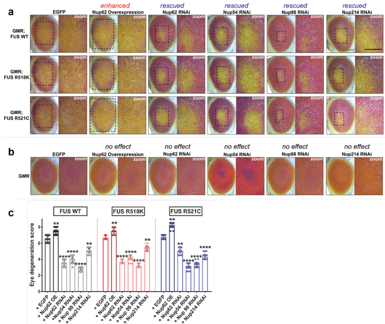
Supplemental Figure 13. Genetic interaction between FUS and nucleoporins in vivo . (a) Representative images of fly eyes showing that modulation of nucleoporins in FUS WT and mutant backgrounds modifies the external eye degeneration caused by FUS expression, indicated by areas of depigmentation and ommatidial fusion. Black dashed boxes highlight areas of marked eye degeneration; the size of the box corresponds to the area of degeneration. Zoom panels are used to further emphasize the extent of eye degeneration. Overexpression of Nup62 (Nup62 OE) enhances external eye degeneration in FUS-expressing flies. Knockdown of Nup62, Nup54, Nup98 and Nup214 rescues the external eye degeneration in FUS-expressing flies. Scale bar= 100µm. (b) Representative images of eye phenotypes of flies overexpressing Nup62 or expressing RNAi for Nup62, Nup54, Nup98, and Nup214 indicates no external eye degeneration caused by modulation of Nup expression. Zoom images show intact and healthy ommatidia. (c) Quantification of eye degeneration (from b) indicates statistically significant difference in eye phenotypes upon modulation of nucleoporins in FUS WT, FUS R518K and FUS R521C backgrounds (n=48 per group). Each point represents one adult fly, Kruskal-Wallis test with Dunn's multiple comparisons test was used for analysis. ****p-value<0.0001; FUS-WT + EGFP vs FUS-WT + Nup62 OE p-value=0.0046; FUS-
