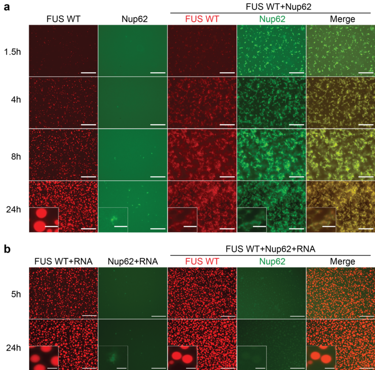
Figure 4. Nup62 and FUS alter the phase separation properties of each other in a manner that is modulated by RNA in vitro . Fluorescence images showing phase separation of 1.5 \mu M MBP-FUS WT (red) doped with \leq 2.5\% Alexa555-labelled MBP-FUS WT and 1.5 \mu M MBP-Nup62 (green) doped with \leq 2.7\% Alexa488-labelled MBP-Nup62. Full-length FUS and Nup62 proteins were used herein. (a) MBP-FUS forms dynamic spherical droplets (Supplemental Video 1). Co-mixing MBP-FUS with MBP-Nup62 promotes the formation of FUS/Nup62-containing amorphous assemblies that appear less dynamic (Supplemental Video 2). (b) Co-mixing as in (a) in the presence of RNA (mass ratio of RNA:FUS:Nup62 \approx 1.5:1:1 ) prevents the formation of amorphous assemblies, giving way to spherical droplets MBP-FUS with some MBP-Nup62 co-localization. Images were taken at the indicated timepoints after initiation of phase
