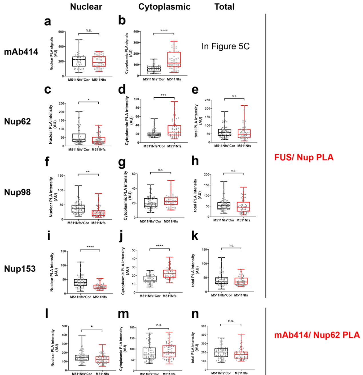
Supplemental Figure 12. Additional PLA data analyses corresponding to Figure 5. (a-k) FUS/Nup PLA. (a, b) FUS/mAb414 PLA. Similar nuclear (a) and a significantly higher cytoplasmic (b) PLA intensity in FUS M511Nfs neurons compared to control neurons. M511Nfs*Cor, n=45; M511Nfs, n=54 cells. n.s.= not significant, ****p<0.0001. (c-e) FUS/Nup62 PLA. A significantly lower nuclear (c), higher cytoplasmic (d) and similar total (e) PLA intensity in FUS M511Nfs neurons compared to control neurons. *p=0.0117, ***p=0.0008; n.s.= not significant. (c) t=2.562, df=112. (d) t=3.455, df=104. M511Nfs*Cor, n=53; M511Nfs, n=53 cells (e) t=0.5965, df=121. M511Nfs*Cor, n=58; M511Nfs, n=65 cells. (f-h) FUS/Nup98 PLA. A significantly lower nuclear (f), similar cytoplasmic (g) and total (h) PLA intensity in FUS M511Nfs neurons compared to control neurons. **p=0.0014,
