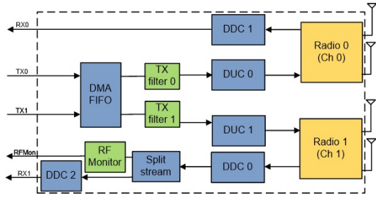
Figure 3: FPGA configuration with dual PHY and RFMON
