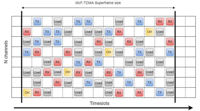
Figure 4: McF-TDMA slot table structure and possible states.
