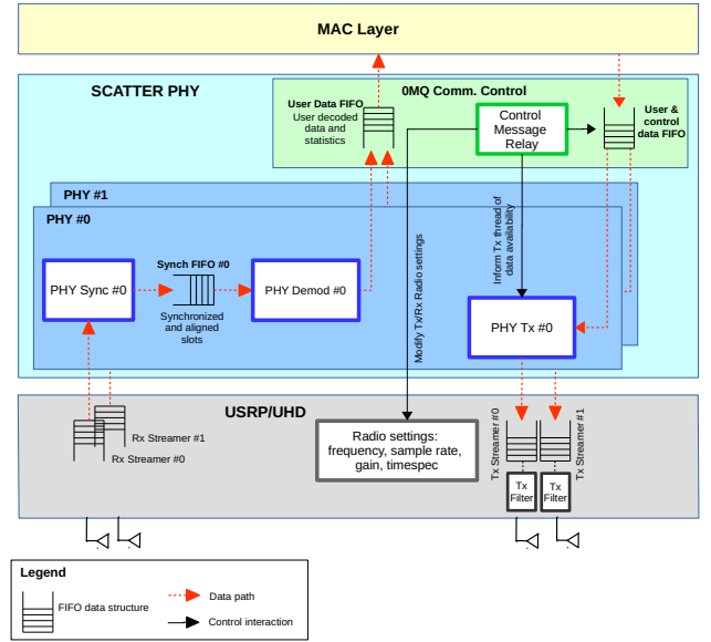
Figure 2: High-level architecture of the SCATTER PHY.
