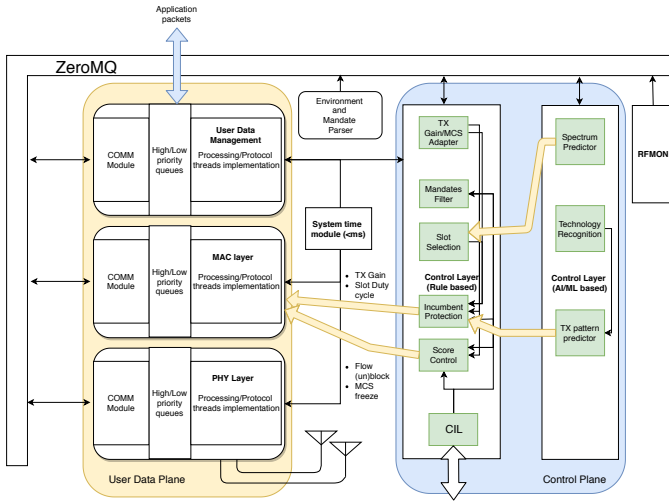
Figure 1: SCATTER system architecture.
