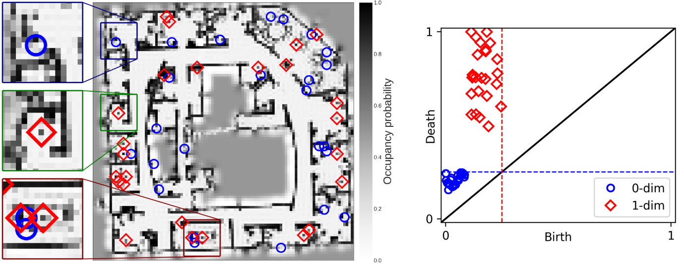
(a) The death locations of the most-persistent topological structures. 0-dim: blue circles; 1-dim: red diamonds. The three cutouts show topologically-challenging regions: (top) a narrow passage connects two parts of a room; (middle) an obstacle lies in the middle of a room; (bottom) a cluttered region consists of several 0-dim and 1-dim structures.
