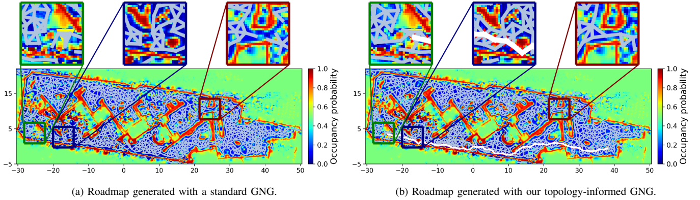
Fig. 4. Two roadmaps generated for the FHW environment. The three cutouts show uncertain narrow passages where the standard GNG in Fig. (a) failed to make a connection and therefore cannot be used for finding paths. Our topology-informed GNG in Fig. (b) biases the sampling towards these challenging regions and therefore can be used to successfully generate a path from one side of the environment to the other (white path).
