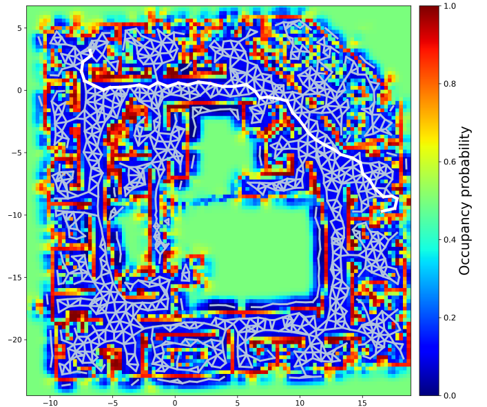
Fig. 1. A roadmap (grey graph) generated by our topology-informed growing neural gas algorithm. The probabilistic occupancy grid (colored image) is generated using a Hilbert map [5] from point-cloud observations of the Intel Research Lab [8]. The white path is a solution path planned over the roadmap through uncertain obstacles and narrow doorways.
