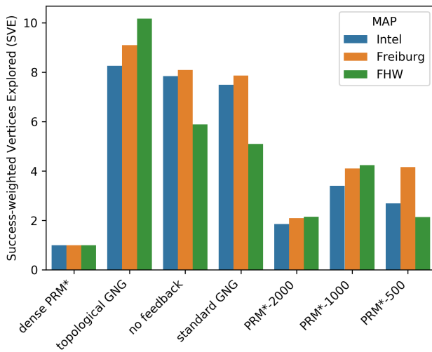
Fig. 7. The success-weighted vertices explored (defined in Sec. V-A3) achieved by the methods. Higher SVE values indicate that the roadmaps are relatively sparse and therefore can be efficiently searched over by Dijkstra's graph search. The baseline dense PRM* performed relatively poorly here due to the increased number of vertices.
