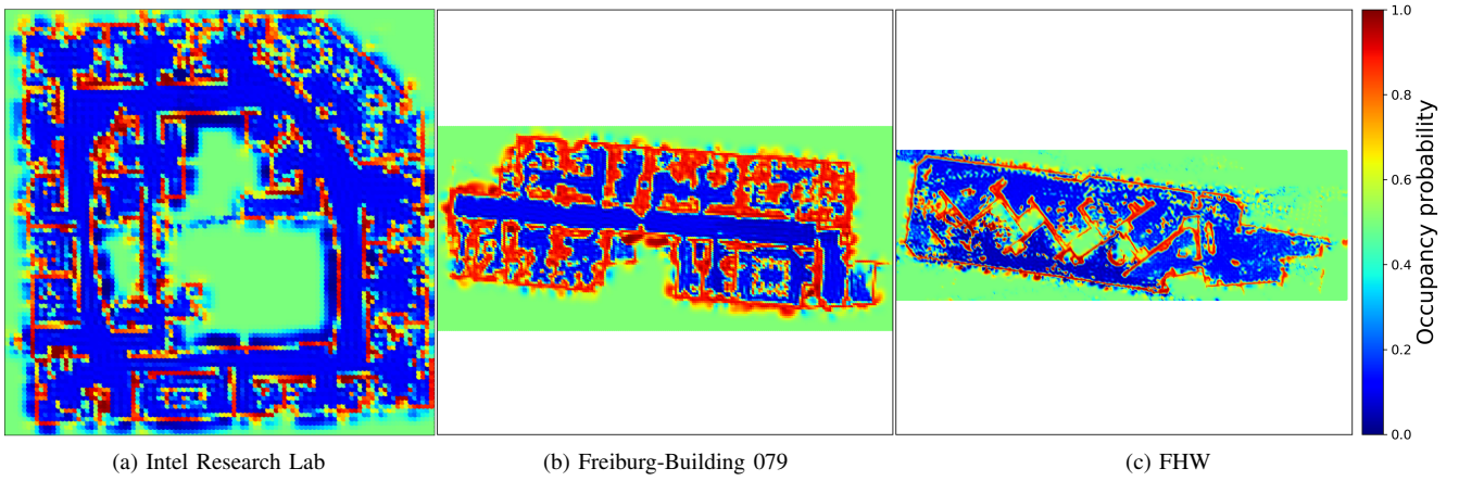
Fig. 3. An illustration of the probabilistic occupancy maps used in the experiments, generated from the point-cloud datasets [8] recorded by robots in three indoor environments and the Hilbert mapping technique [5]. The environments have varying configurations of rooms, doorways, narrow passages, and noisy obstacles, and are between 20 m and 80 m across.
