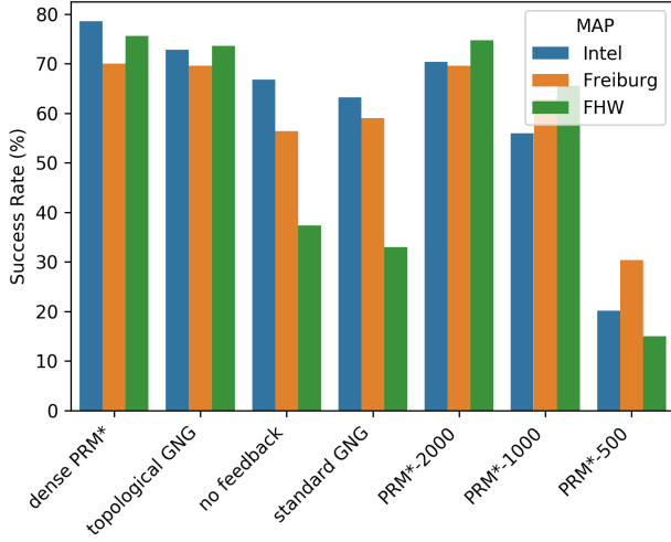
Fig. 5. The success rate achieved by the comparison methods for 500 start-goal pairs in the three maps of Fig. 3. Higher success rates indicate the roadmap has good connectivity across the environment. Our topological GNG achieves a similar success rate to dense PRM* and enables much more efficient search (see Fig. 7).
