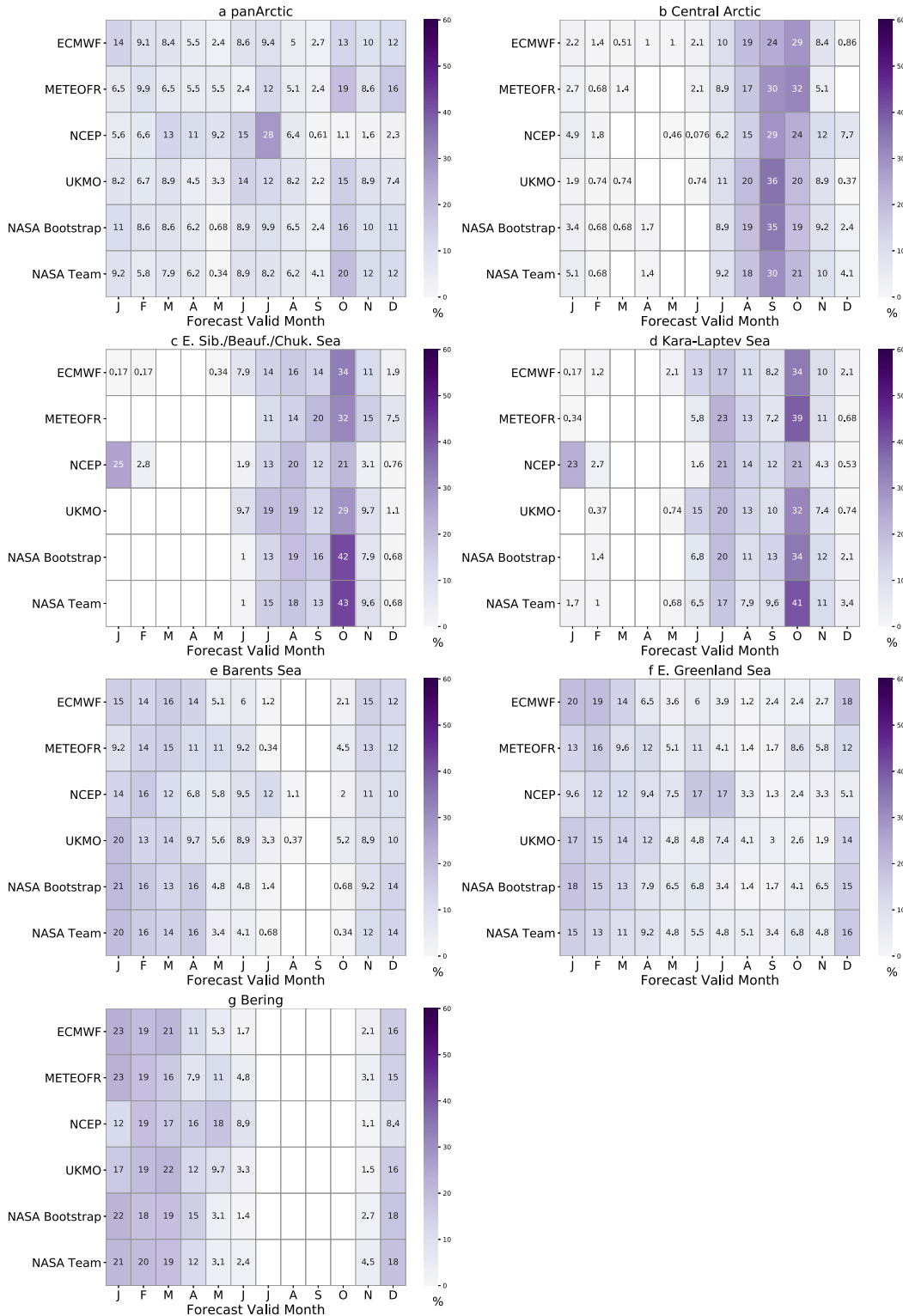
FIG. 8. As in Fig. 7, but with VRILE days calculated based on the bottom 5th percentile of the 5-day change in anomalous sea ice extent.
