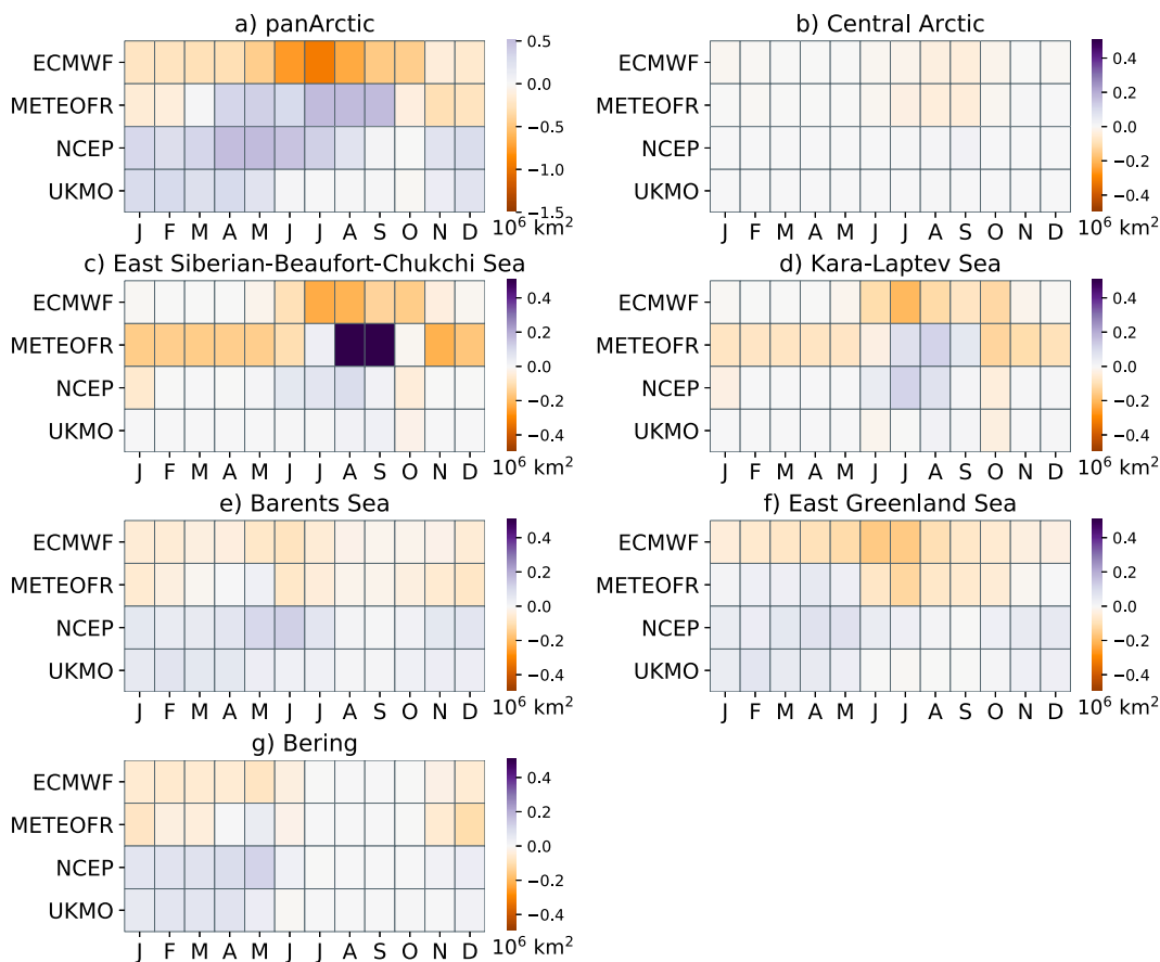
FIG. 4. Bias ( SIE_{\text{model}} - SIE_{\text{obs}} ) in predictions of sea ice extent as a function of forecast valid month. Bias is calculated for lead days 0–1, relative to the NASA Bootstrap observations.
