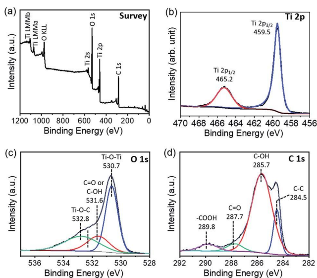
Fig. 3 XPS spectra of TiO 2 -short SWCNT. (a) XPS survey spectrum; deconvolution of high-resolution Ti 2p spectrum (b), O 1s spectrum (c), and C 1s spectrum (d).
