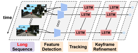
Fig. 1: Learning monocular visual odometry with long-term modeling. Existing self-supervised methods only see short snippets during the training time, which makes it hard to learn to leverage temporal consistency over long sequences. Our method, in contrast, inspired by geometry-based visual odometry methods, combines the best of both the geometry and learning to aggregate long-term temporal information.
