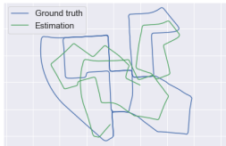
(a) SfMLearner [53]
