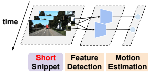
Fig. 1: Learning monocular visual odometry with long-term modeling. Existing self-supervised methods only see short snippets during the training time, which makes it hard to learn to leverage temporal consistency over long sequences. Our method, in contrast, inspired by geometry-based visual odometry methods, combines the best of both the geometry and learning to aggregate long-term temporal information.
