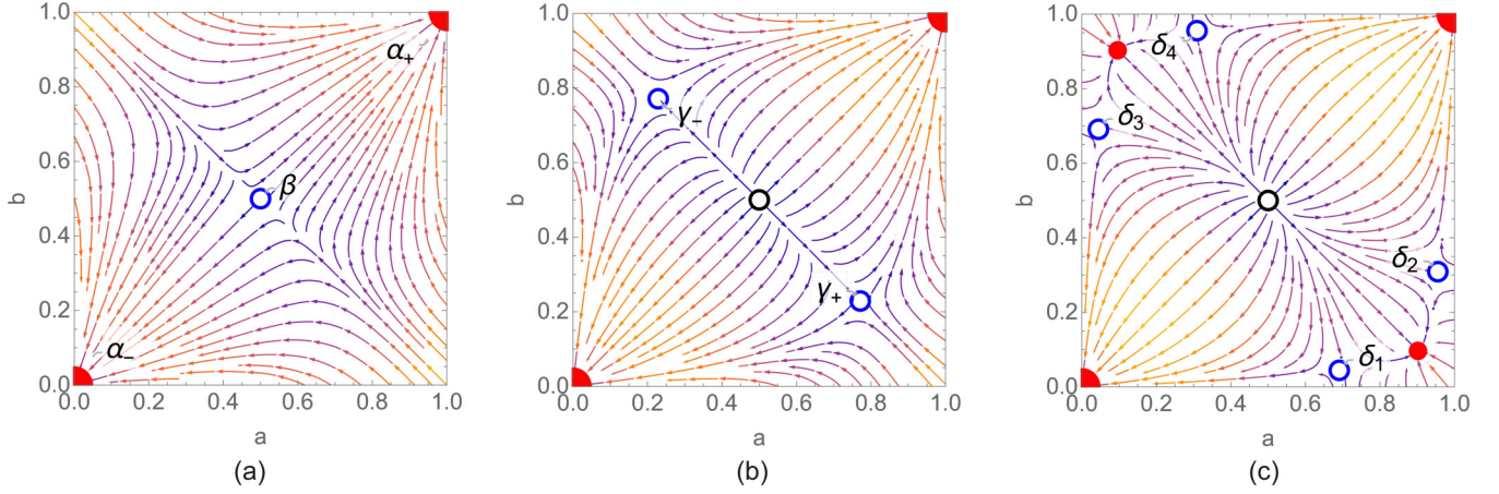
FIG. 1. Flow field of the dynamical system defined by Eq. (1) for the cases: (a) \epsilon = 0.25 (greater than \epsilon^c = \frac{1}{3} ), (b) \epsilon = 0.15 (between \epsilon_c = \frac{1}{9} and \epsilon^c ), and (c) \epsilon = 0.08 (less than \epsilon_c ). The arrow colors indicate the flow magnitude [blue (darker) slow, red (lighter) fast] and the symbols indicate the locations of the fixed points: red dots for stable, blue circles for saddles, and the black circle at (\frac{1}{2}, \frac{1}{2}) in (b) and (c) for unstable.
