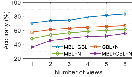
Fig. 15. Accuracy in multi-view multiple-distortions scenario. With six views aggregated, the accuracy can improve by 9.3% to 19.4% given different distortion combinations.
