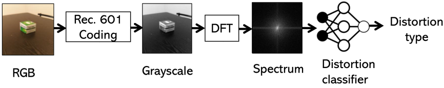
Fig. 7. The pipeline of the image distortion classification. The Fourier spectrum is used as the input of the distortion classifier for training and classification.
