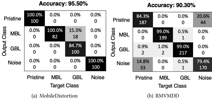
Fig. 10. Confusion matrix and accuracy of the image distortion classifier on different datasets: (a) MobileDistortion and (b) RMVMDD. On average, the distortion classifier achieves 95.5% and 90.3% accuracy on the two datasets, respectively.
