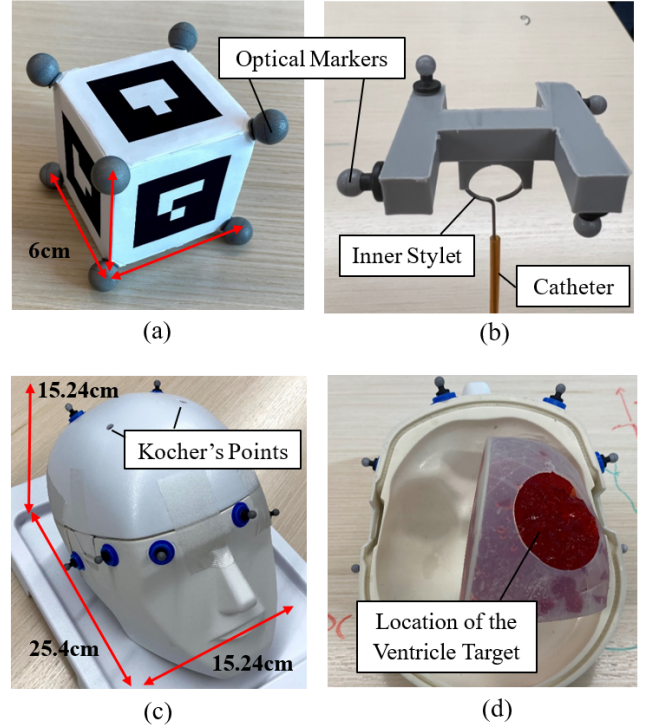
Figure 2: (a) 3D printed localization marker attached with both fiducial (ARToolKit) and optical markers. (b) H-shaped 3D printed mount for the catheter, attached to the inner stylet. (c) Dimensions of the phantom model attached with eight optical markers and Kocher’s points. (d) A mold filled with jello inside the phantom model.
