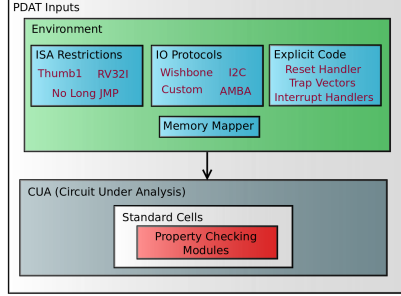
Fig. 3. A component-diagram of the PDAT input.
