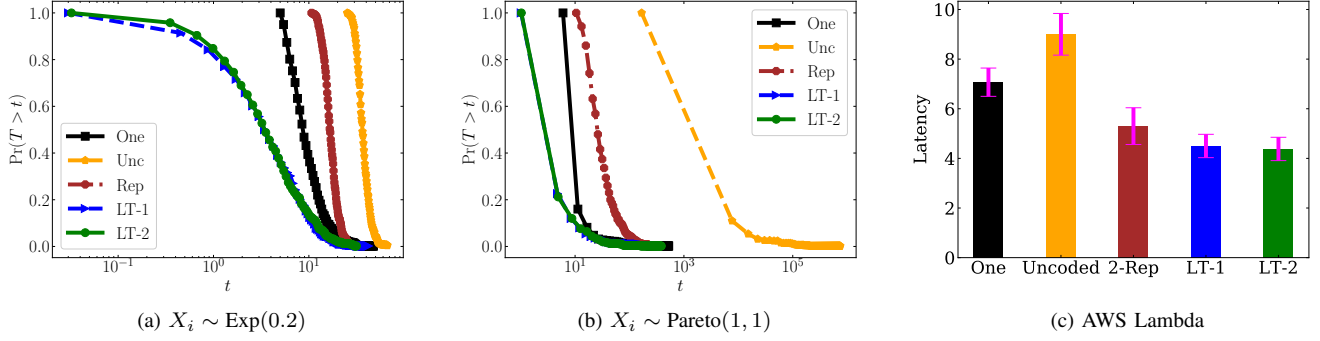
Fig. 2: The tail probability of the latency is the highest for the Uncoded scheme for both \text{Exp}(0.2) and \text{Pareto}(1,1) distributions on initial delay X_i . Observe that One (All-at-One) where the entire computation is performed by a single node is faster than Uncoded in all cases, and also has a lighter tail than 2-Replication in the simulations ((a) and (b)). Both LT coded schemes, LT-1 and LT-2, have the lightest latency tail probability in the simulations and are the fastest in the AWS Lambda experiments. Both simulations and experiments use m = 1000 .
