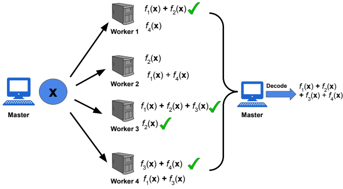
Fig. 1: An illustration of our rateless coded (LT-1) strategy for a system of 4 workers tasked with computing F(x) = \sum_{i=1}^4 f_i(x) . Tick marks indicate completed tasks which suffice to recover F(x) . Observe that Worker 2 (straggler) does not complete any tasks.
