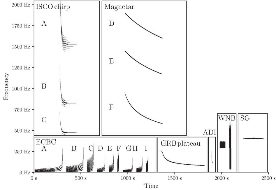
FIG. 1. Time-frequency spectrogram of the reference waveforms used in this search. We show examples of astrophysical waveforms such as postmerger magnetars (Magnetar) [22], black hole accretion disk instabilities (ADI) [18], newly formed magnetar powering a gamma-ray burst plateau (GRB plateau) [16], eccentric inspiral-merger-ringdown compact binary coalescence waveforms (ECBC) [23], broadband chirps from innermost stable circular orbit waves around rotating black holes (ISCO chirp) [12], and “ ad hoc ” waveforms, band-limited white noise burst (WNB) and sine-Gaussian bursts (SG). The ISCO chirp waveforms have been shifted up in frequency by 50 Hz for readability. Durations range from 6 (ADI-B) to 470 s (GRB plateau).
