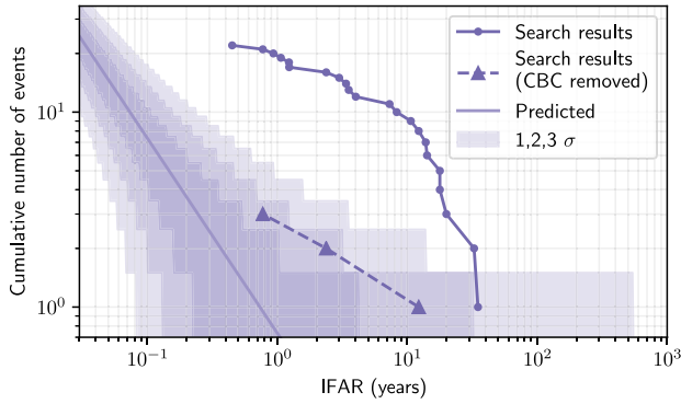
FIG. 4. Cumulative number of events versus IFAR found by the BW follow-up to the CWB low-frequency analyses using all O3 data (circular points) and after times around all compact binary coalescence sources have been excised (triangular points). The solid line shows the expected background, given the analyzed time. The shaded regions show the 1, 2, and 3 \sigma Poisson uncertainty regions.
