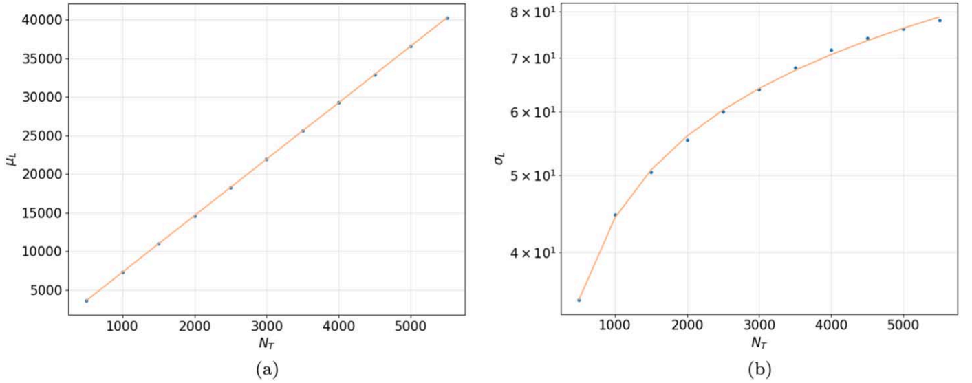
Figure 9. (a) Mean \mu_L and (b) standard deviation \sigma_L of the log-likelihoods of the Viterbi paths as a function of N_T . Blue circles are values obtained from 100 trials of simulations. The orange curves are the linear and power-law fits describing the mean and standard deviation dependence on N_T . An analogous calibration is presented in Millhouse et al. (2020).
