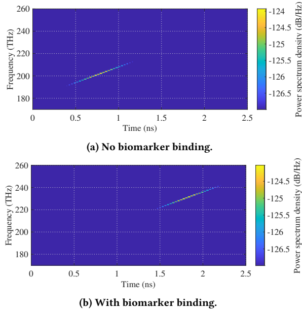
Figure 11: Detection of antenna resonant frequency before and after binding based on the cutoff frequency and power spectrum.
