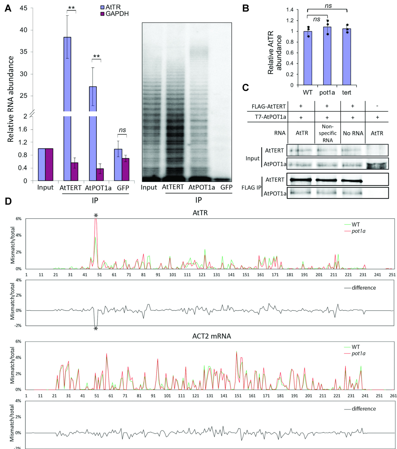
Figure 1. AtPOT1a does not engage Arabidopsis telomerase via interaction with AtTR. (A), qPCR (left) and TRAP (right) results from immunoprecipitated samples to measure the copurification of AtTR (left), GAPDH mRNA (left) and active telomerase (right). Anti-AtTERT and Anti-GFP IPs served as positive and negative controls, respectively. Error bars indicate standard deviation. ** P value < 0.01 and ns (not significant) were calculated based on Student's t -test. (B) qPCR results for AtTR in wild-type (WT), tert and pot1a mutants. A single data point represents an individual biological repeat. Error bars indicate standard deviation. ns was calculated based on Student's t -test. (C) In vitro co-IP experiments performed in a coupled transcription/translation system in the presence or absence of different RNA molecules. Co-purification of AtPOT1a was measured after Anti-FLAG IP. (D) In vivo chemical probing of RNA secondary structure by targeting specific DMS-MaPseq from WT Arabidopsis and pot1a mutants. Average mutation frequencies from two biological replicants are plotted along AtTR and ACT2 mRNA sequences separately. Asterisk (*) denotes the template region of AtTR with increased flexibility in the pot1a mutant.
