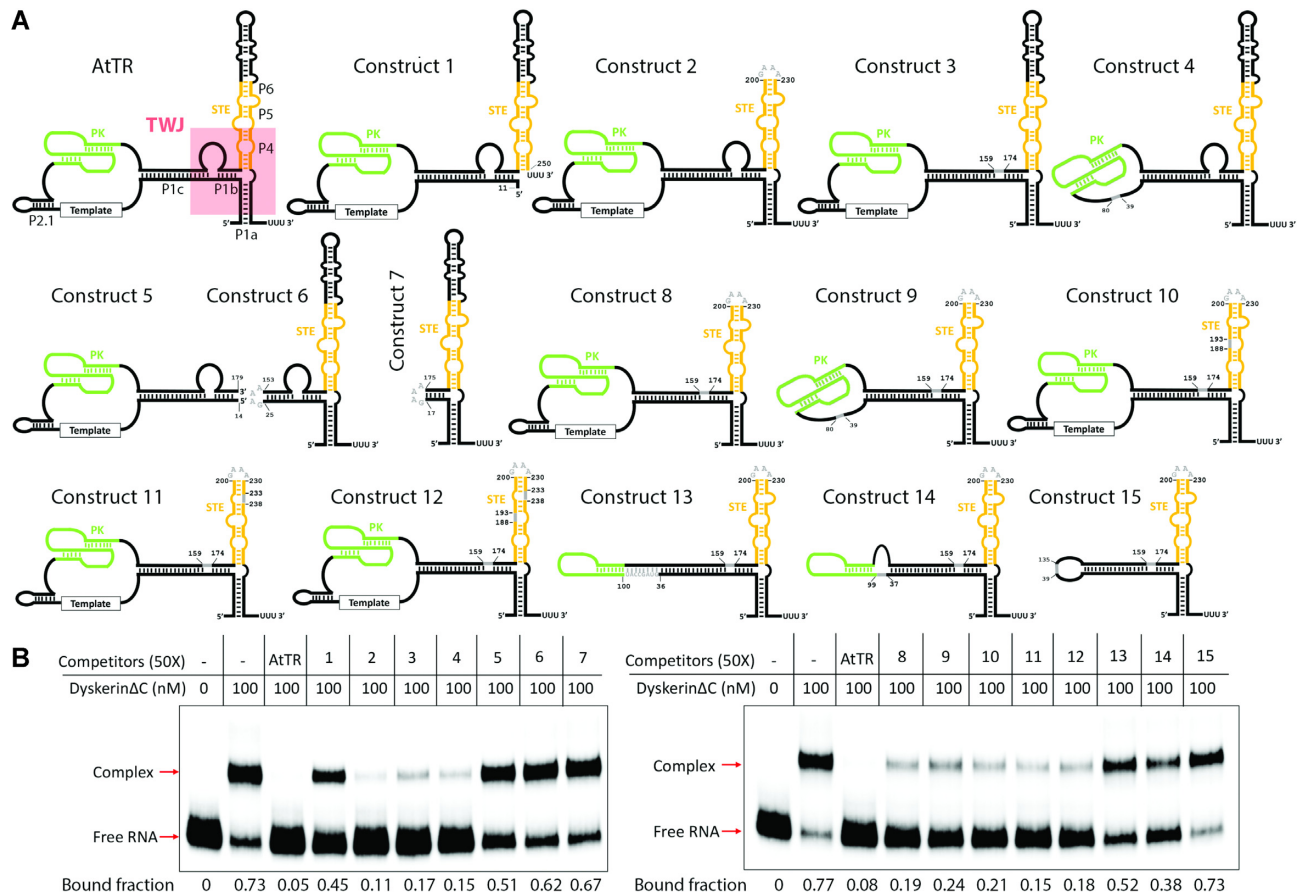
Figure 3. Mapping the dyskerin binding site on AtTR. (A) Secondary structures of WT AtTR and constructs 1–15. (B) Competitive EMSA performed with 50X excess non-radiolabeled AtTR or individual truncations. Signal intensities were quantified to calculate the bound RNA fraction. Mutation constructs 2, 3, 4, 8, 9, 10, 11 and 12 show strong competition; construct 14 shows moderate competition; constructs 1, 5, 6, 7, 13 and 15 show weak competition or no competition.
