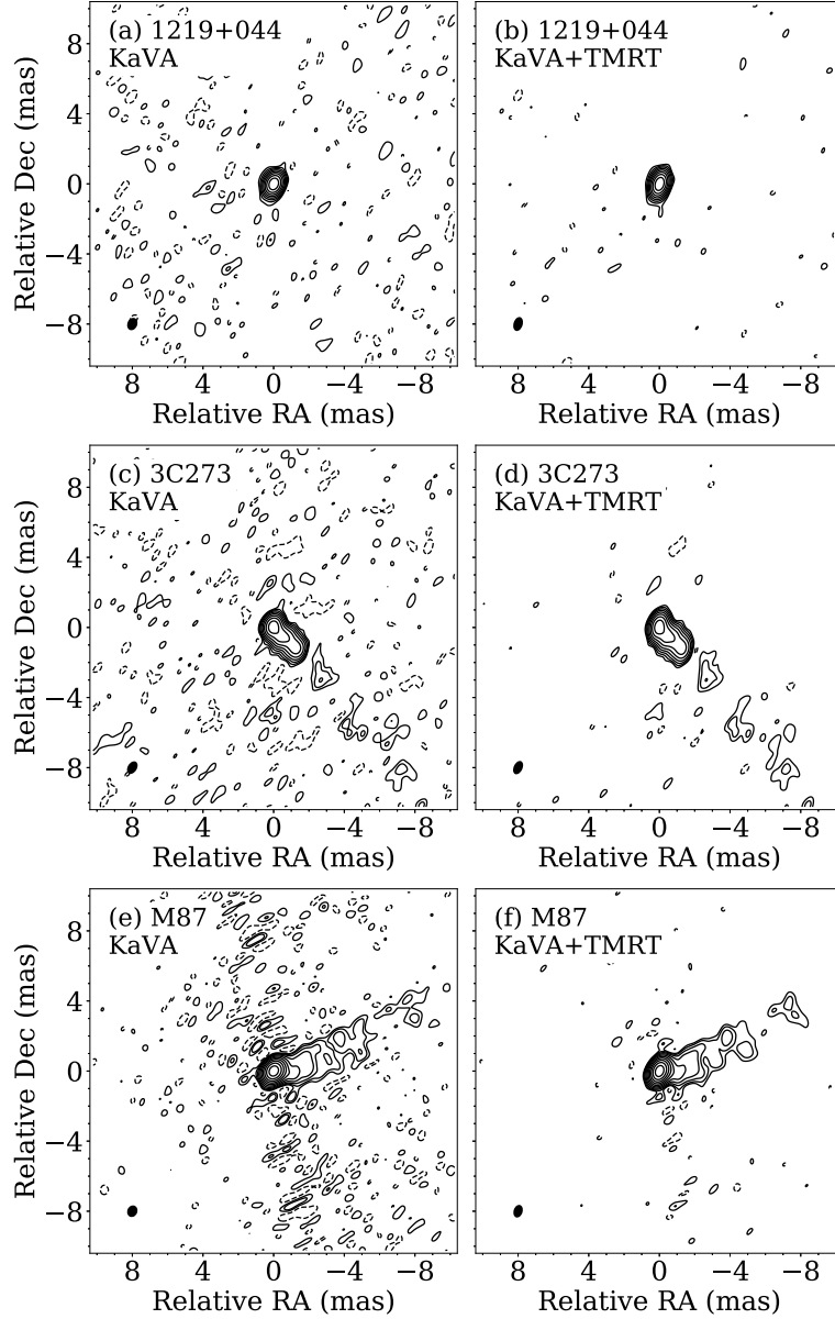
Fig. 7: Structure images of 1219+044 (a, b), 3C 273 (c, d) and M 87 (e, f): KaVA (a, c, e) and KaVA+TMRT (b, d, f) in Session-Q. The first contour is consistent in all images for the same source, namely 3.04 mJy/beam for 1219+044, 20.19 mJy/beam for 3C 273, 1.49 mJy/beam for M 87. The increase steps are (-1, 0, 1, 1.4, 2, 2.8...). A synthesized beam is indicated in the bottom-left corner of each panel.
