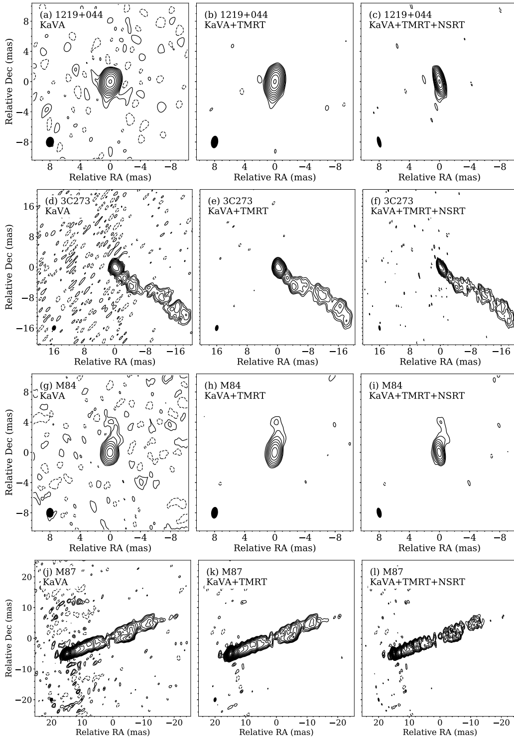
Fig. 6: Structure images of 1219+044 (a-c), 3C 273 (d-f), M87 (g-i) and M84 (j-l): KaVA ( left ), KaVA+TMRT ( middle ) and KaVA+TMRT+NSRT ( right ) in Session-K. The first contour is consistent in both images for the same source, namely 1.02 mJy/beam for 1219+044, 9.32 mJy/beam for 3C 273, 1.20 mJy/beam for M87, 1.37 mJy/beam for M84. The increase steps are (-1, 0, 1, 1.4, 2, 2.8...). A synthesized beam is indicated in the bottom-left corner of each panel.
