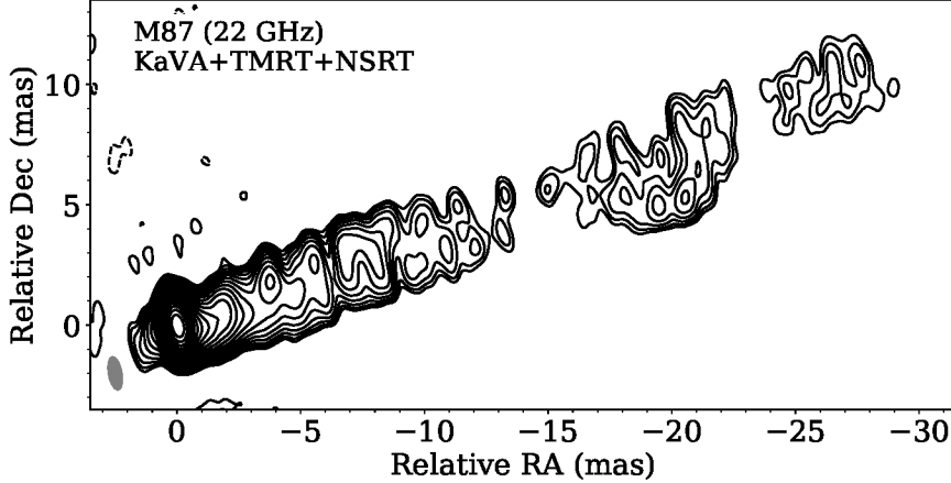
Fig. 9: KaVA+TMRT+NSRT image of M87 in Session-K covering the whole jet up to \sim 30 mas from the core. Contour levels are scaled as (-1, 0, 1, 1.4, 2, 2.8, \dots) \times 1.20 mJy/beam. The synthesized beam is shown in the bottom-left corner of the figure.
