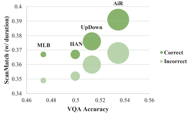
Figure 4. Comparison of VQA models’ answer accuracy, scanpath accuracy, and machine attention accuracy (bubble size).
