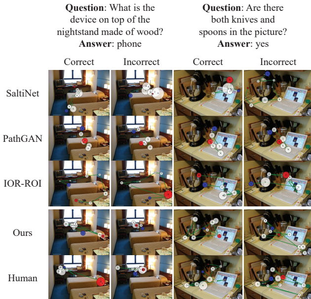
Figure 3. Examples of the predicted scanpaths. Each column compares the prediction results and human scanpaths given specific answer correctness. The number and radius indicate the fixation order and duration, respectively. The blue and red dots indicate the beginning and the end of the scanpath, respectively.
