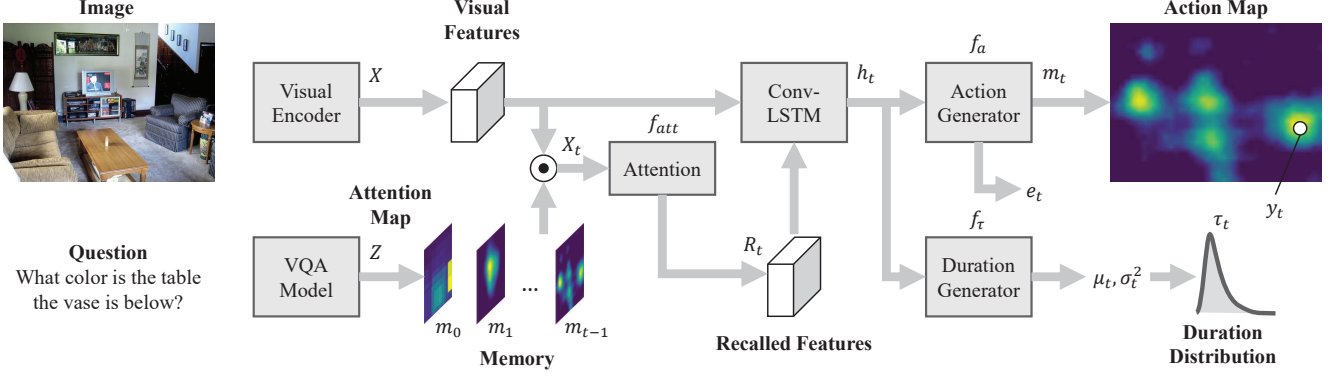
Figure 2. Overview of the proposed scanpath prediction network.
