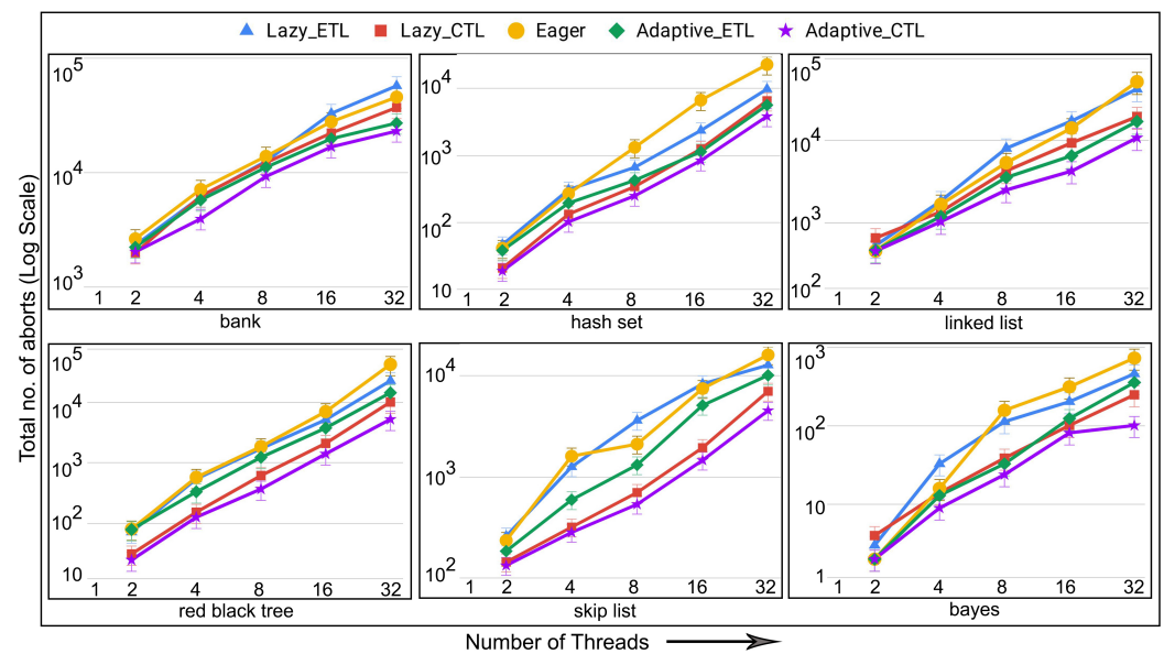
Figure 20. Number of aborts in micro-benchmarks and bayes from STAMP using better time barrier in non-persistent TM.
