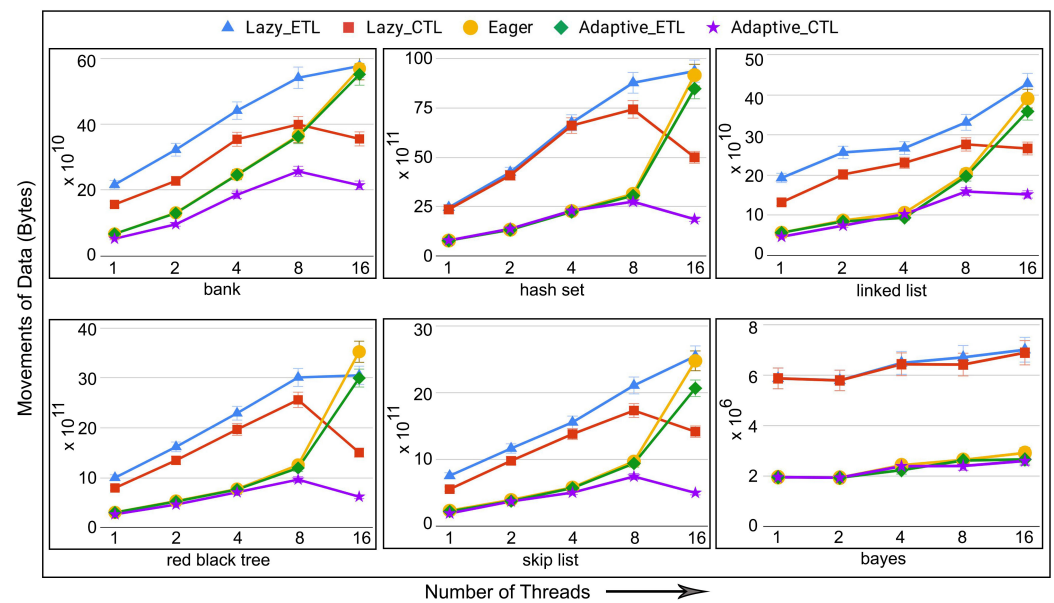
Figure 7. Data movements in micro-benchmarks and bayses from STAMP executing in persistent TM.
