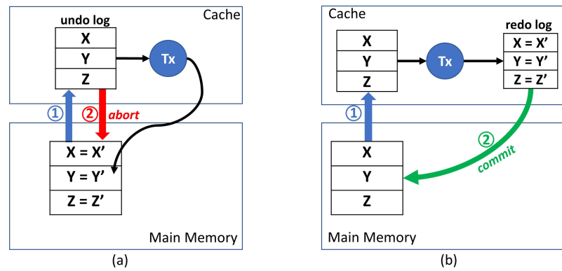
Figure 2. An illustration of how a transaction T_x is executed in non-persistent memory using (a) eager versioning and (b) lazy versioning. Figure (a) depicts two kinds of operations in eager versioning. The first operation is to copy the data from original memory locations to a log area (called undo log ) in cache. Transaction T_x then performs in-place updates to the original memory locations. Now, the second operation is to copy the data back from the log area to the original memory locations, in case T_x aborts. If T_x commits, the data in the log area is simply discarded. Figure (b) depicts two kinds of operations in lazy versioning. The first operation is to copy the data from original memory locations to a log area (called redo log ) in cache. Transaction T_x updates on this redo log. Then, the second operation is to copy updated data from the log area to the original memory locations, in case T_x commits. If T_x aborts, the data in the log area is simply discarded.
