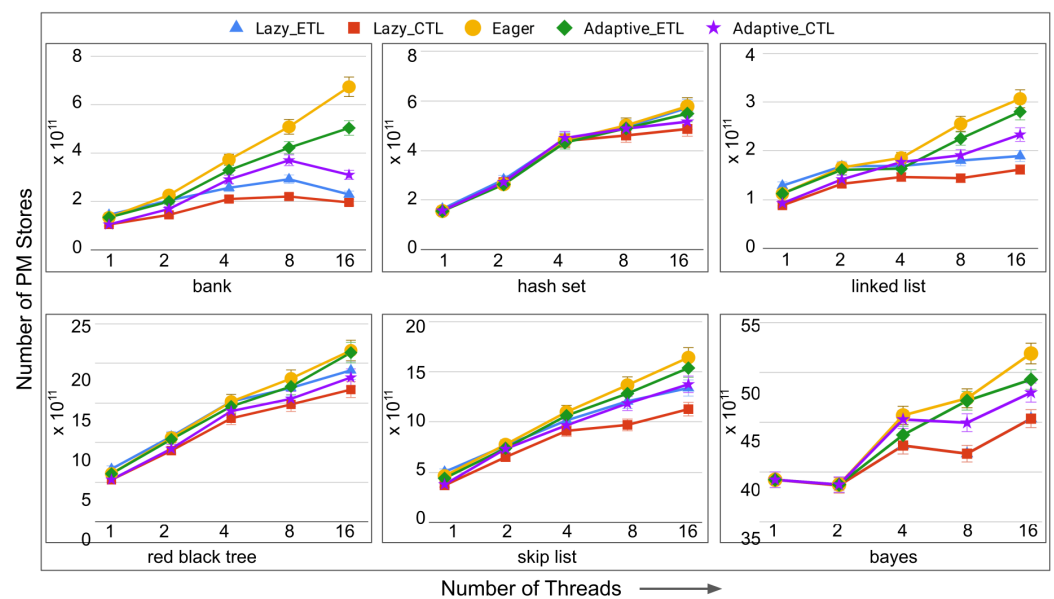
Figure 8. Total number of stores to the PM in micro-benchmarks and bayses from STAMP.
