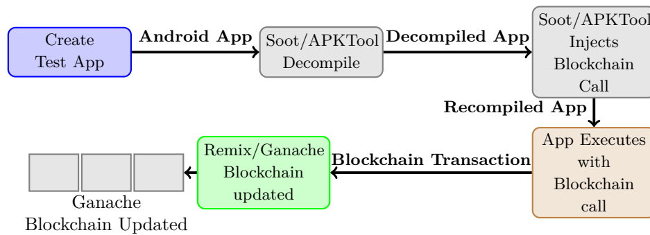
Figure 3. Overview of code injection
