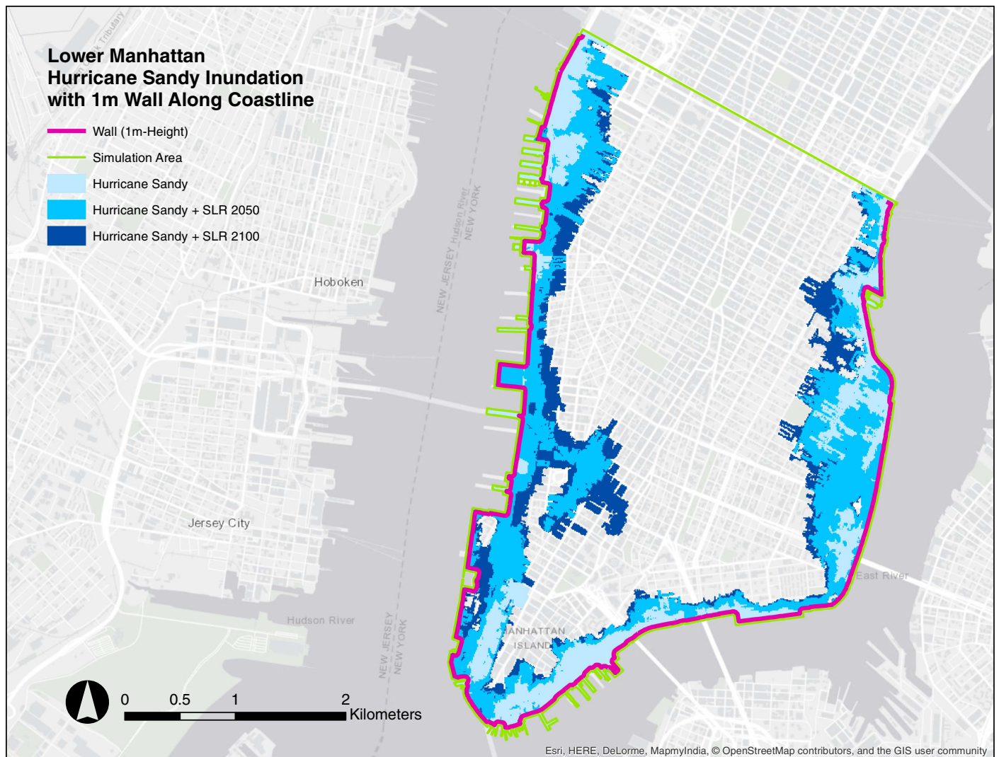
Fig. 14. Results for extent of flooding obtained using proposed GISSR methodology for following three scenarios: Hurricane Sandy, Hurricane Sandy plus SLR middle estimate in 2050s, and Hurricane Sandy plus SLR middle estimate in 2100. The following protective measure is considered: seawall of height 1 m along entire length of coastline of Lower Manhattan (bold line on map). (Base map by Esri, HERE, DeLorme, MapmyIndia, © OpenStreetMap contributors, and the GIS user community.)
