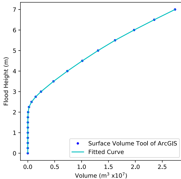
Fig. 5. Flood height estimation curve for Division 12 in Fig. 2. The data points computed by ArcGIS's Surface Volume tool are fitted with the square root function in Eq. (8).
