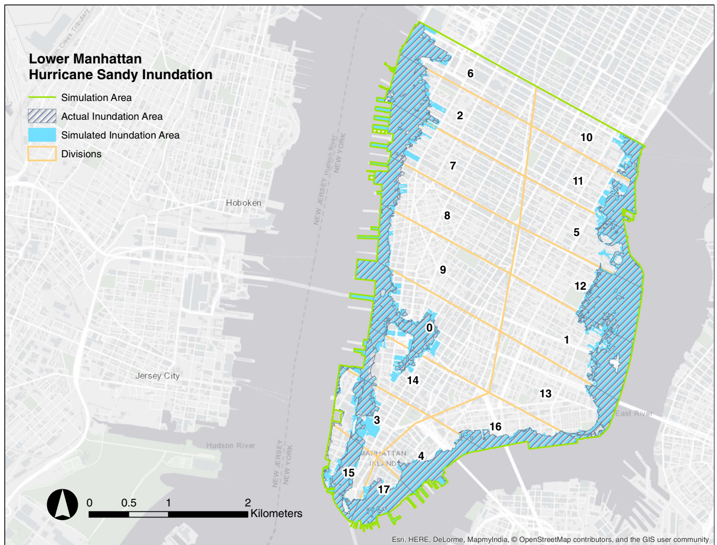
Fig. 8. Actual flooded area during 2012 Hurricane Sandy versus corresponding results obtained using proposed GISSR methodology. (Base map by Esri, HERE, DeLorme, MapmyIndia, © OpenStreetMap contributors, and the GIS user community.)
