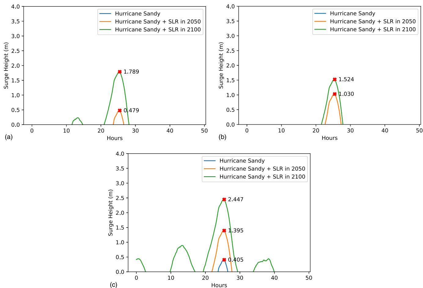
Fig. 16. Time histories of floodwater height at the three locations. At each location, three scenarios are considered: Hurricane Sandy, Hurricane Sandy plus SLR middle estimate in 2050s, and Hurricane Sandy plus SLR middle estimate in 2100. The following protective measure is considered: seawall of height 1 m along entire length of coastline of Lower Manhattan: (a) South Ferry subway station; (b) Canal Street subway station; and (c) Con Edison Plant at 14th St.
