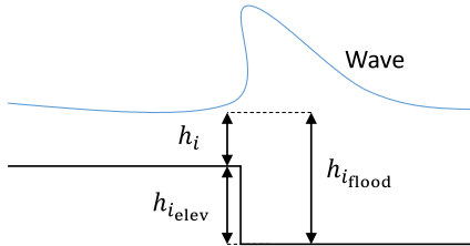
Fig. 4. Definitions and relationship between h_i(t) , h_iflood(t) , and h_ielev .
