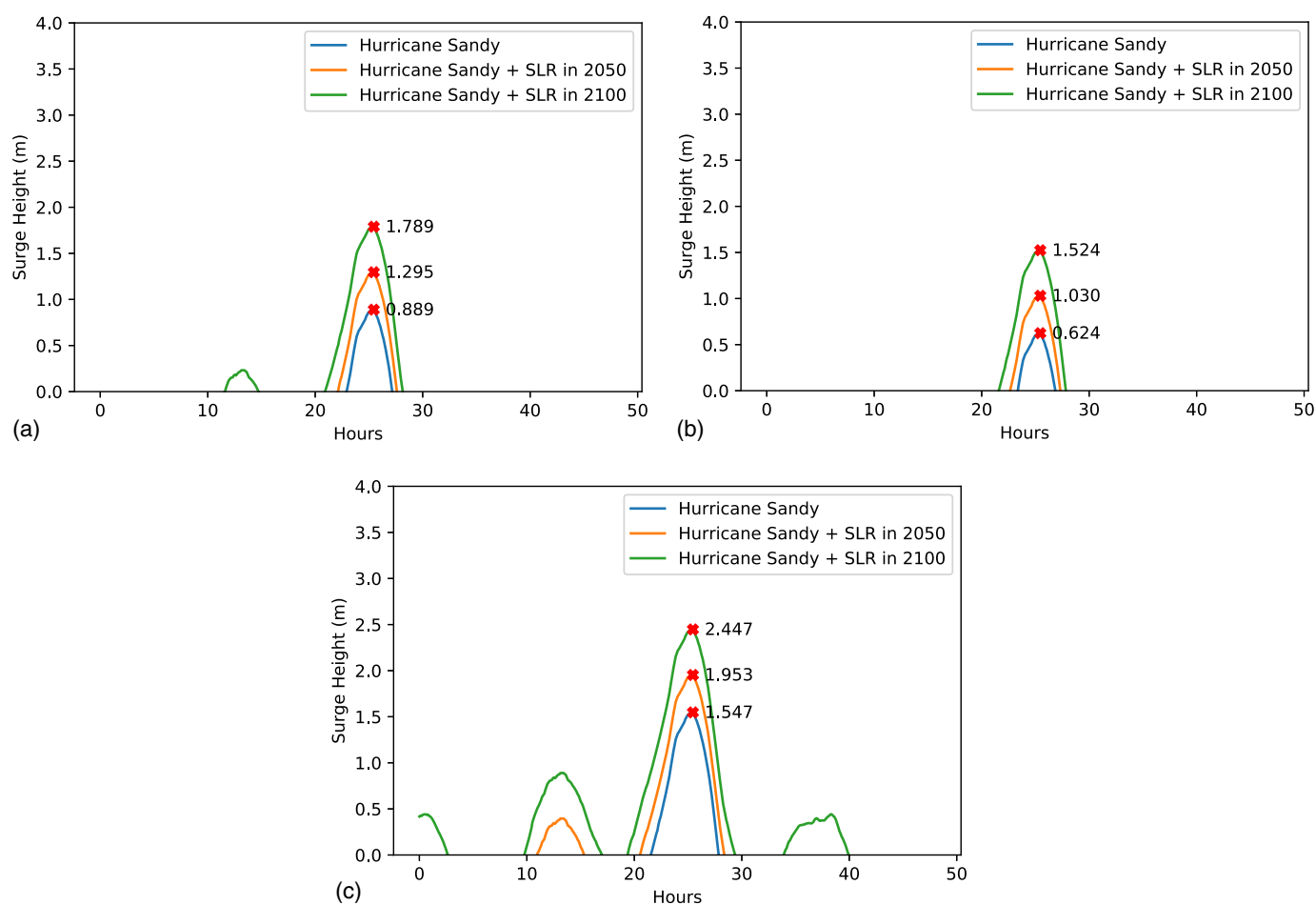
Fig. 10. Time histories of floodwater height at following locations: (a) South Ferry subway station entrance (latitude: 40.7013, longitude: -74.0135 ); (b) Canal Street subway station entrance on Seventh Avenue (40.7208, -74.0054 ); and (c) Con Edison Power Plant at East 14th Street (40.727835, -73.973181 ). At each location, three scenarios are considered: Hurricane Sandy, Hurricane Sandy plus SLR middle estimate in 2050s, and Hurricane Sandy plus SLR middle estimate in 2100. No protective measures are considered in these simulations: (a) South Ferry subway station; (b) Canal Street subway station; and (c) Con Edison Plant at 14th St.
