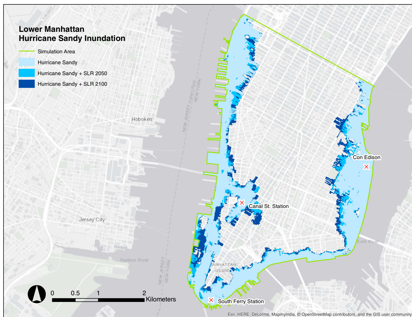
Fig. 9. Results for extent of flooding obtained using proposed GISSR methodology for following three scenarios: Hurricane Sandy, Hurricane Sandy plus SLR middle estimate in 2050s, and Hurricane Sandy plus SLR middle estimate in 2100. No protective measures are considered in these simulations. (Base map by Esri, HERE, DeLorme, MapmyIndia, © OpenStreetMap contributors, and the GIS user community.)
