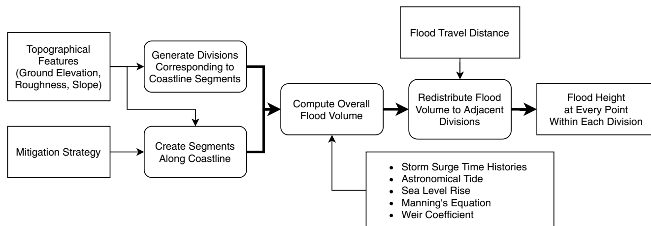
Fig. 1. Flood simulation schematic diagram; rectangles: inputs, rounded rectangles: processes.
