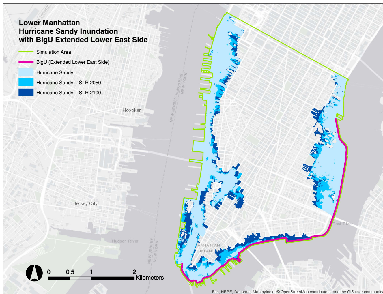
Fig. 13. Results for extent of flooding obtained using proposed flood simulation methodology for following three scenarios: Hurricane Sandy, Hurricane Sandy plus SLR middle estimate in 2050s, and Hurricane Sandy plus SLR middle estimate in 2100. The following protective measure is considered: seawall of height 4.57 m (15 ft) along length of Compartments C1–C3 (bold line on map). (Base map by Esri, HERE, DeLorme, MapmyIndia, © OpenStreetMap contributors, and the GIS user community.)
