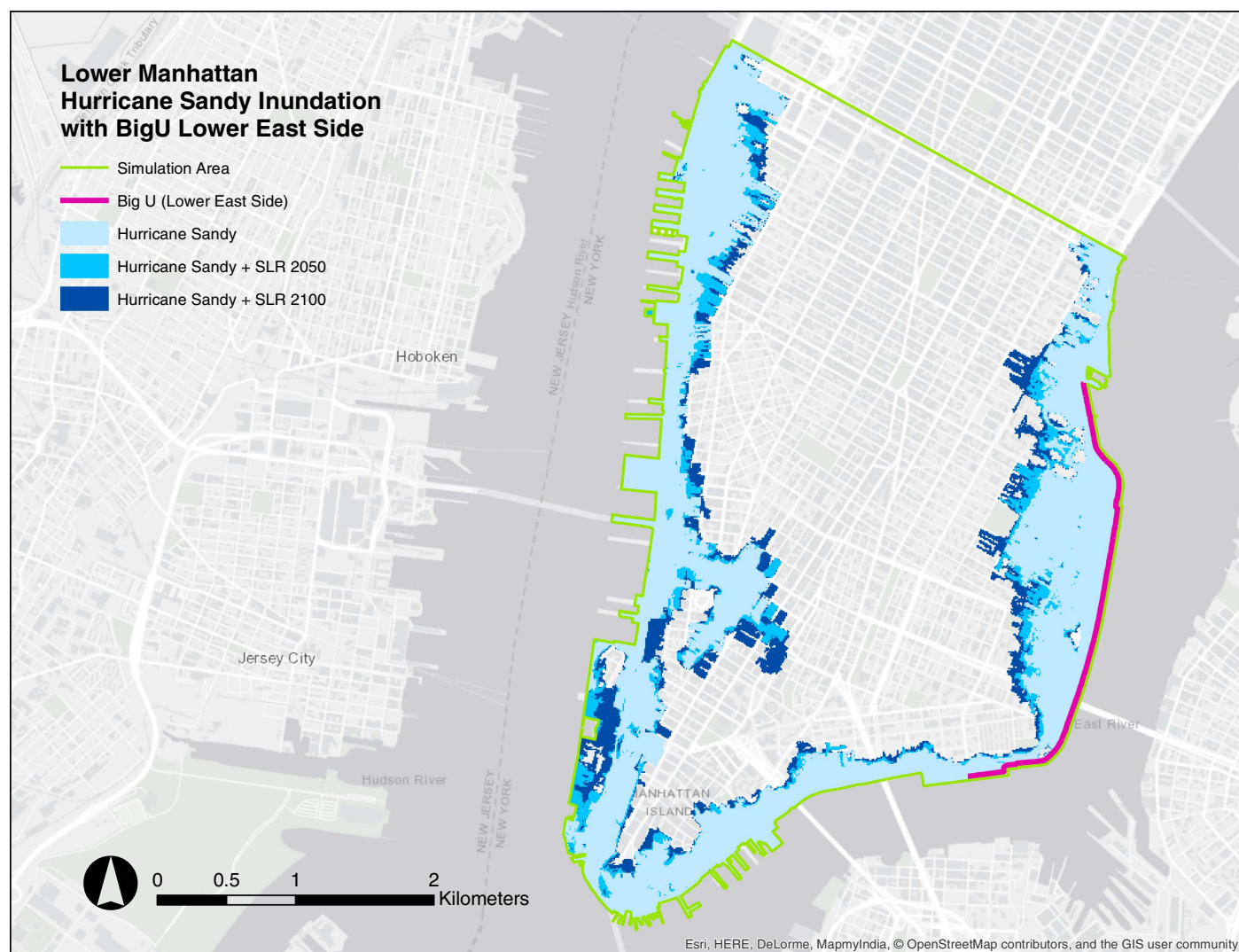
Fig. 12. Results for extent of flooding obtained using proposed GISSR methodology for following three scenarios: Hurricane Sandy, Hurricane Sandy plus SLR middle estimate in 2050s, and Hurricane Sandy plus SLR middle estimate in 2100. The following protective measure is considered: seawall of height 4.57 m (15 ft) along length of Compartment C1 (bold line on map). (Base map by Esri, HERE, DeLorme, MapmyIndia, © OpenStreetMap contributors, and the GIS user community.)
