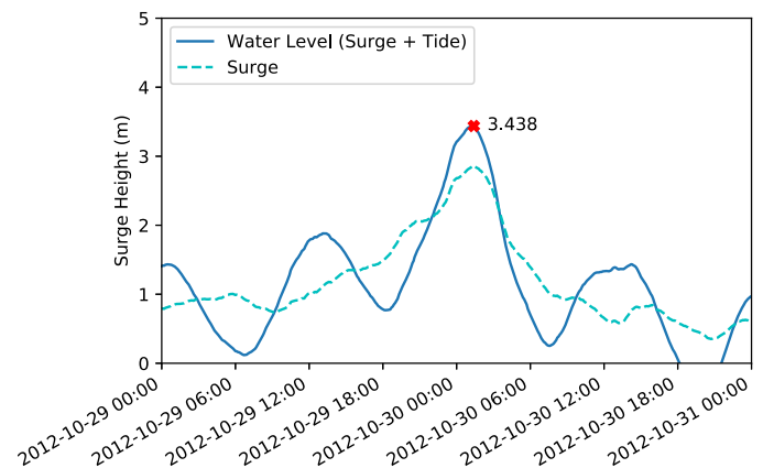
Fig. 7. Time history of total water level (storm surge + tide) observed at Battery in Manhattan (Station 8518750) during Hurricane Sandy. The number of data points is 480. (Data from National Oceanic and Atmospheric Administration 2012.)
