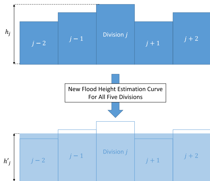
Fig. 6. Schematic of floodwater transfer/exchange among adjacent divisions for the case of two divisions on each side of a given division j . The new flood height estimation curve used is established for all five divisions considered as a single division in the figure. The total water volume in the divisions remains the same, satisfying the conservation of mass.
