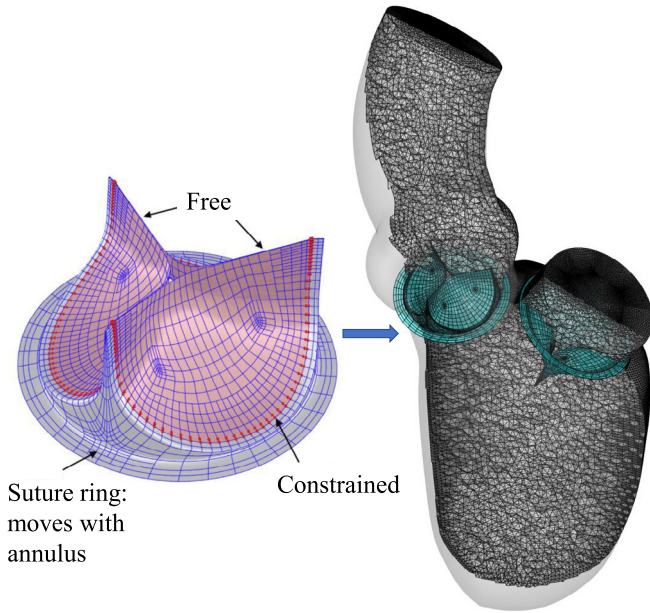
Fig. 2. The BHV model discretization and configuration of the AV and MV implants, which are immersed into the LV fluid domain. The control points with constrained motion are highlighted by red color in the left-hand-side figure. (For interpretation of the references to color in this figure legend, the reader is referred to the web version of this article.)
