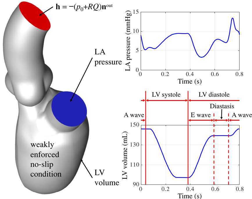
Fig. 3. Setup for the FSI simulation. Different phases of the cardiac cycle are labeled on the LV volume curve.
