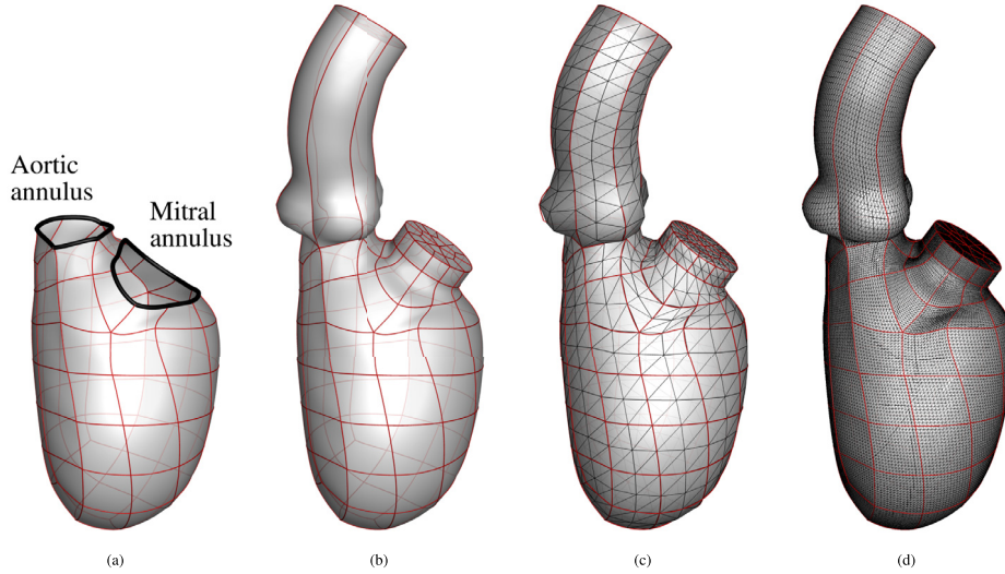
Fig. 1. Reference fluid domain mesh generation: (a) the spline patches making up the left ventricle model; (b) LV model with an idealized aorta and LA extension; (c) coarse triangulation of the model; (d) fine triangulation of the model that is used as the resolution in the FSI simulation.
