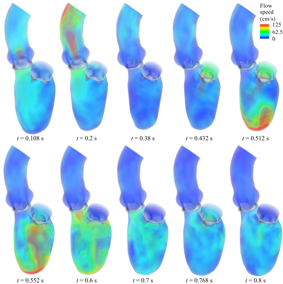
Fig. 4. Visualization of the FSI results for the flow field in the LV and the BHV motions in a complete cardiac cycle.
