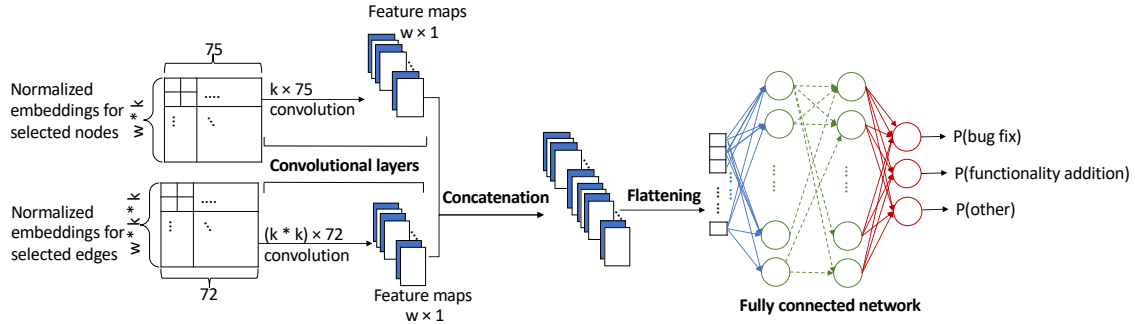
Fig. 6: Overview of CClassifier's CNN structure
