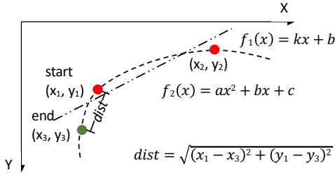
Fig. 4: Tactic inference from any \langle \text{context}, \text{action} \rangle pair
