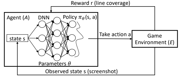
Fig. 15: Overview of RLT—a testing tool based on RL
