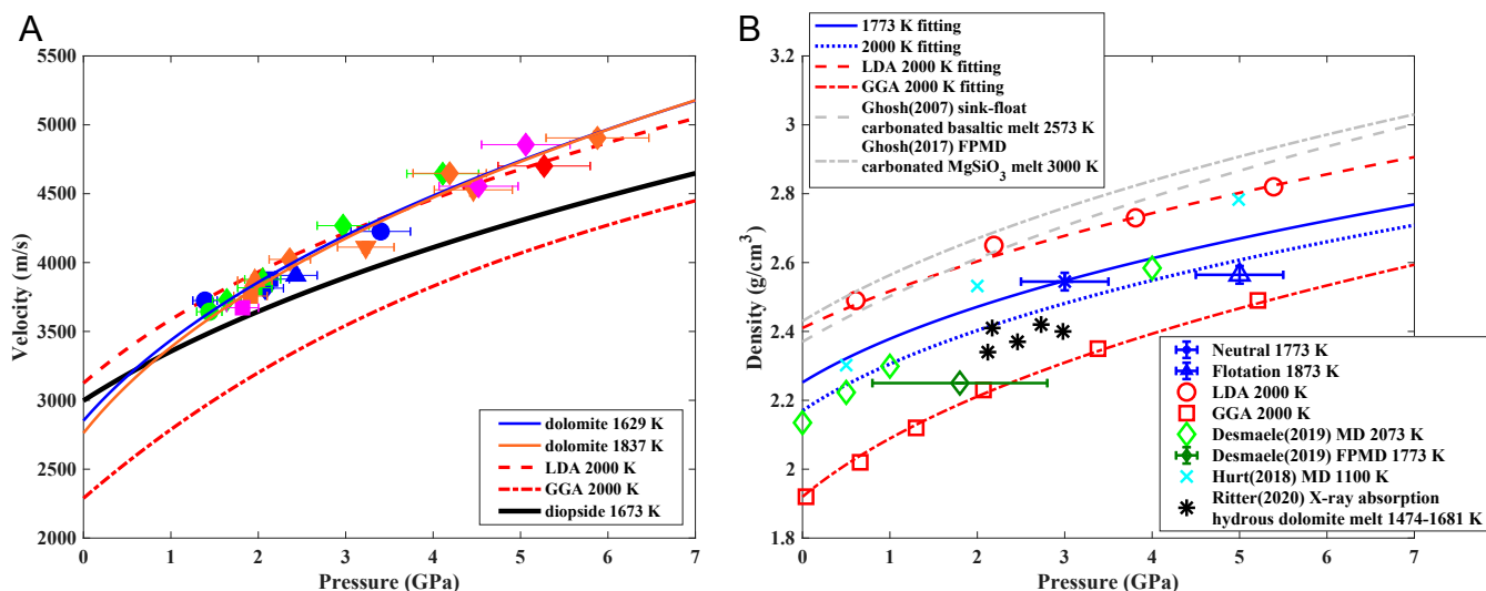
Fig. 2. (A) Sound velocity as a function of pressure for dolomite melt. Different markers correspond to different experimental runs: square-T2207, circle-T2208, upward-pointing triangle-T2261, downward-pointing triangle-T2262, diamond-T2439. Different marker colors correspond to different temperatures: blue-1629 K, green-1733 K, orange-1837 K, magenta-1942 K, red-2046 K. The blue and orange curves are fitted velocity results of dolomite melt along the 1629 K and 1837 K isotherms, respectively. The dashed and dash-dot curves are our FPMD results for dolomite melt along the 2000 K isotherm based on LDA and GGA, respectively. The thick black curve is the velocity profile for diopside melt from Xu et al. (28) for comparison. The diopside melt velocity is calculated along its adiabat with a potential temperature of 1673 K, but the temperature effect on the velocity of diopside melt at high pressures is negligible (28). (B) Density as a function of pressure for dolomite melt obtained from experiments and FPMD simulations in this study, and comparison with previous studies. Blue asterisk-neutral point, blue upward-pointing triangle-flotation point, blue solid line-EOS fitting based on experimental data at 1773 K, blue dotted line-EOS fitting at 2000 K, red circle-density data obtained by LDA, red square-density data obtained by GGA, red dashed line-EOS fitting at 2000 K for LDA, red dash-dot line-EOS fitting at 2000 K for GGA, green diamond-classical MD simulations data at 2073 K from Desmaele et al. (23), cyan cross-classical MD simulations data at 1100 K from Hurt (26), black star-density data of hydrous dolomite melt (with 10 wt% \text{H}_2\text{O} ) at 1474–1681 K from Ritter et al. (35) measured by X-ray absorption method, gray dashed line-density of carbonated basaltic melt (with 5.0 wt% \text{CO}_2 ) from sink-float experimental results by Ghosh S. et al. (36), gray dash-dot line-density of carbonated \text{MgSiO}_3 melt (with 5.2 wt% \text{CO}_2 ) from FPMD results by Ghosh D.B. et al. (37).
