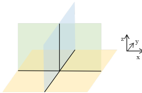
Figure 14: The minimal structure of an X-cube model with rough boundaries.
