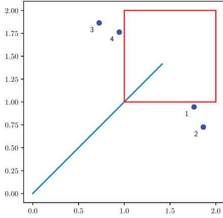
Fig. 3: 1R planar arm, and estimates of end-effector collisions.
