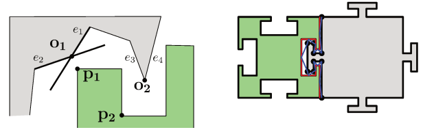
(a) The edge-vertex distance constraints limit the valid motions in a small convex region. (b) The distance constraints generated for a pair of rigid bodies. Blue line segments are vectors from green vertices to red edges.
