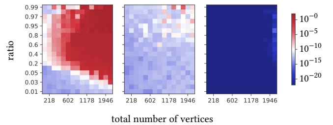
Fig. 21. Heatmap showing the final error \|\hat{\Theta} - \Theta\|_\infty for spheres of varying resolution (x-axis) with some ratio (y-axis) of the vertices set to target angle 3 and the rest to a constant target angle < 2\pi such that the Gauss-Bonnet theorem is satisfied. Left: double precision results when the two angle values are distributed in two clusters. Center: double precision results when the two angle values are distributed randomly over the sphere. Right: extended precision (150 bits mantissa) results with the same distribution as left. (For this experiment, the threshold for the gradient norm decrease was set to 0 and, to reduce the run time in this particular case, \lambda was chosen adaptively, initially halved until the range of coefficients of \lambda d was less than 10.)
