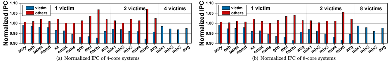
Figure 3: Normalized Performance overhead of IVcache when fixing 1, 2, or all running benchmark(s) as the victim(s).
