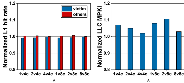
Figure 5: Average cache performance. N_1VN_2C means the systems with N_1 victim(s) and N_2 cores.
