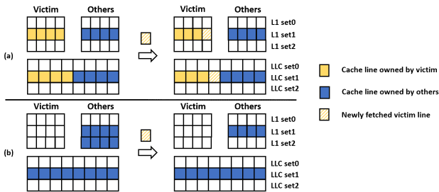
Figure 1: (a) Self-eviction and (b) Bypass mechanism; L1 cache is bypassed in (b) due to cache inclusion.
