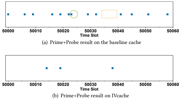
Figure 4: Prime+Probe attack results.
