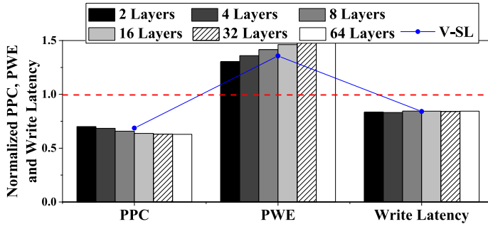
Fig. 27. Results of PPC, PWE, and Write Latency of RSS-RAID in ideal case and RSS-RAID w/V-SL.
