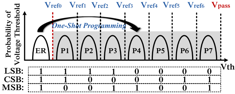
Fig. 2. The voltage distribution of TLC [15, 45].
