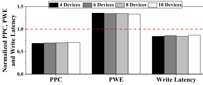
Fig. 28. Normalized PPC, PWE, and Write Latency on RSS-RAID w/V-SL system with different number of SSD devices.
