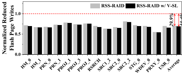
Fig. 24. Normalized PPC decreases of RSS-RAID and RSS-RAID w/V-SL.
