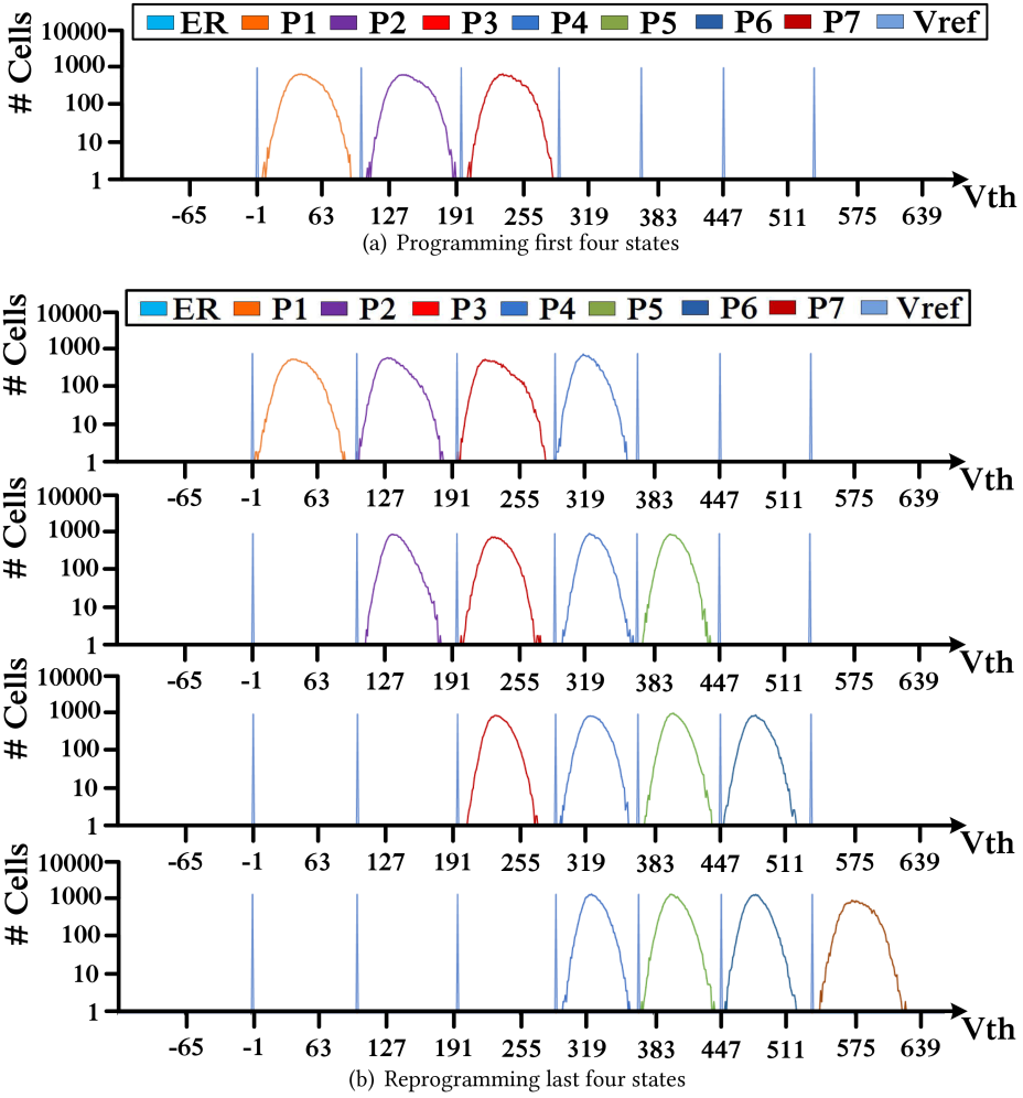
Fig. 4. Voltage distribution after implementing OLR.
