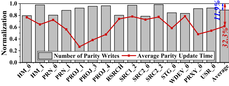
Fig. 10. Normalized number of parity writes and average parity update time.
