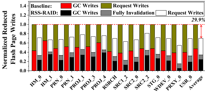
Fig. 13. Normalized physical flash page decrease.
