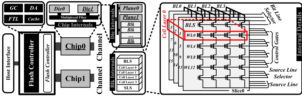
Fig. 1. The architecture of 3D SSD.
