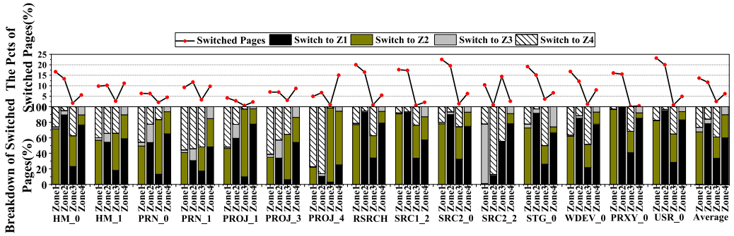
Fig. 26. The percentages of switched pages among four zones.
