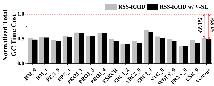
Fig. 14. Normalized total GC time cost.
