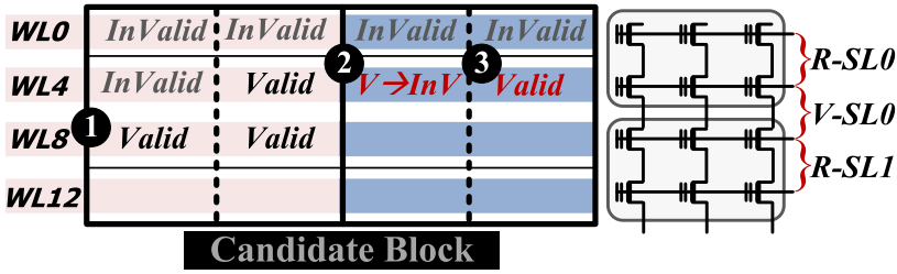
Fig. 12. Reprogramming flash cells across R-SLs.
