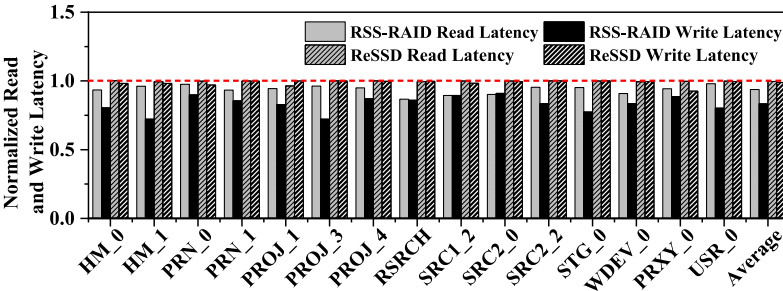
Fig. 21. Normalized read/write latency of RSS-RAID and ReSSD.
