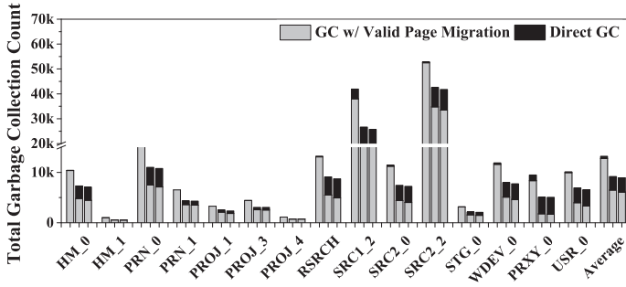
Fig. 25. The number of GCs of baseline, RSS-RAID and RSS-RAID w/V-SL.
