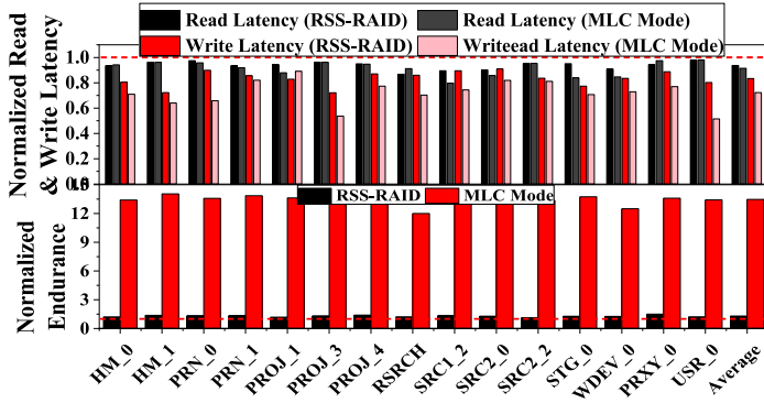
Fig. 22. Comparison among baseline, MLC mode RAID and RSS-RAID.
