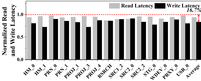
Fig. 17. Normalized read/write latency of RSS-RAID.
