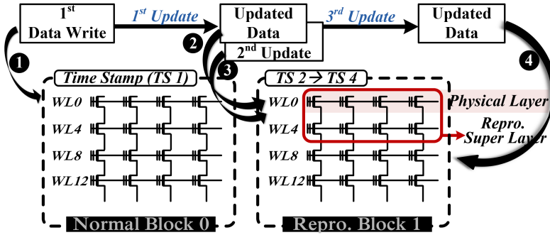
Fig. 7. Hotness based data reprogramming.
