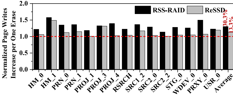
Fig. 20. Normalized number of PWEs of RSS-RAID and ReSSD.
