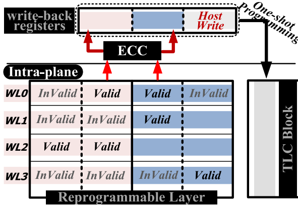
Fig. 9. Migrating valid pages to a normal TLC block accompanied with host write requests.
