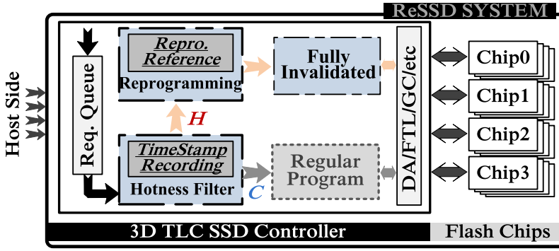
Fig. 6. The overview of ReSSD system design.
