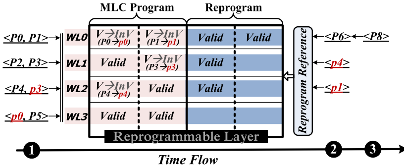
Fig. 8. An example of implementing reprogram operation on R-SL.
