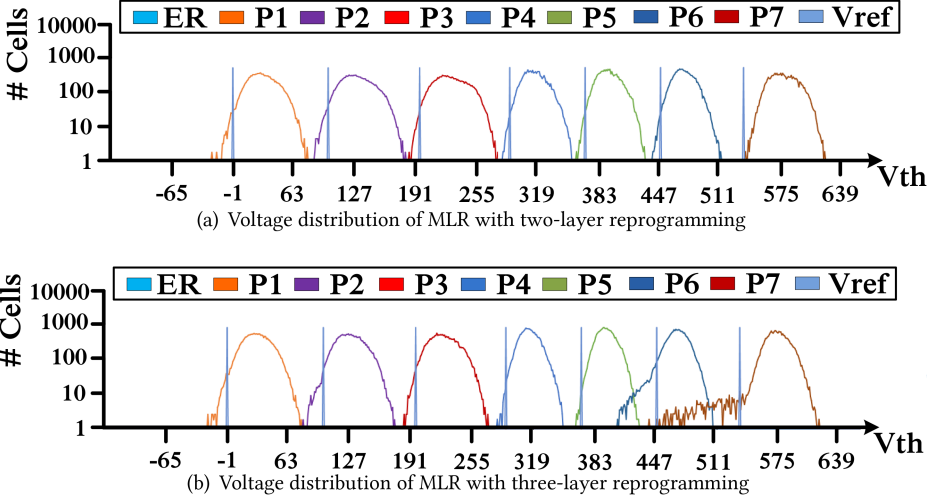
Fig. 5. Worst cases of voltage distributions with implementing MLRs.
