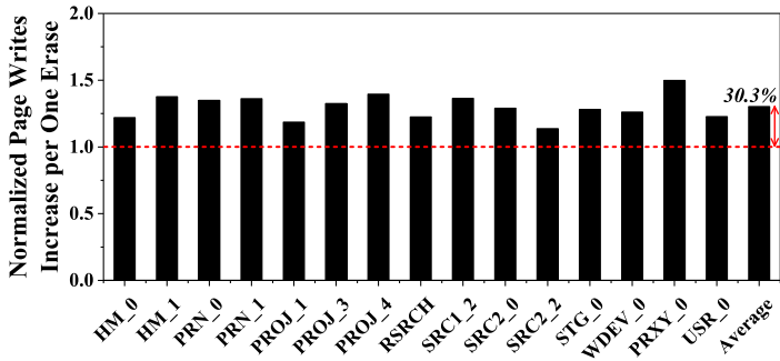
Fig. 16. The number of PWE of RSS-RAID.
