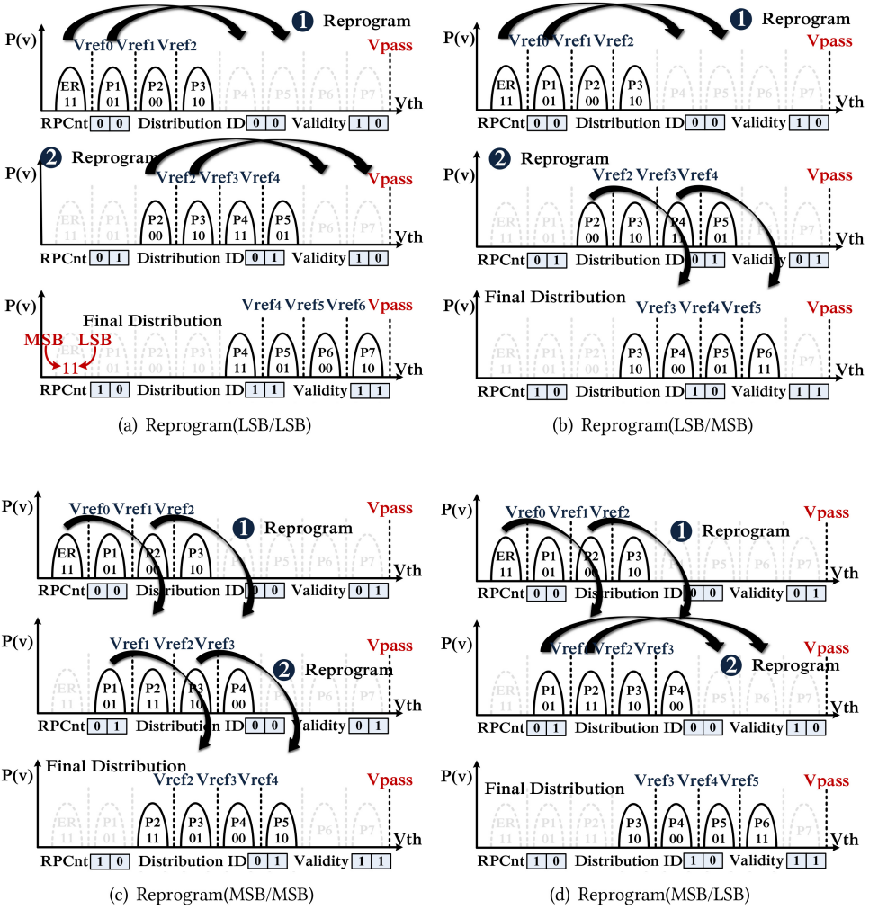
Fig. 3. State movements and voltage distribution arrangements. Reprogram( LSB/MSB ) means the LSB of a MLC mode cell is reprogrammed first, followed by reprogramming the MSB.
