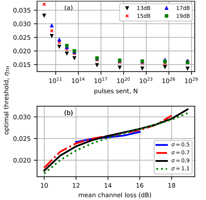
FIG. 1. Simulations. (a) The optimal transmittance threshold, for different number of sent pulses N and for different mean channel losses. Here, \sigma = 0.9 for all simulation points. (b) The optimum threshold in terms of the mean channel loss for different \sigma values. Here, N = 3 \times 10^{10} for all simulation points.
