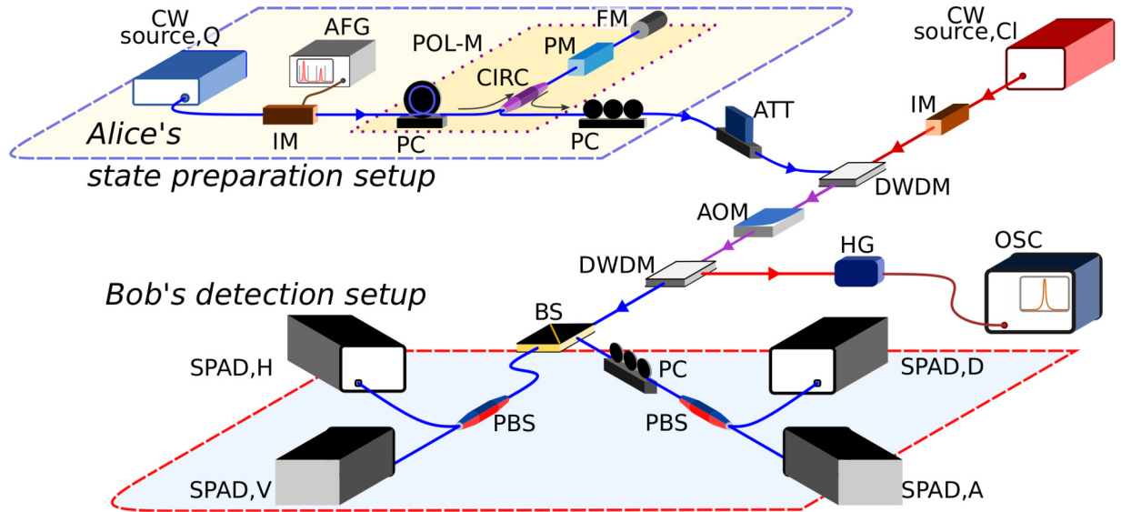
FIG. 2. A continuous-wave source (CW source, Q) is used to encode the quantum states on. Pulses are carved with an intensity modulator (IM) driven by an arbitrary function generator (AFG). The driving voltage sequence contains three voltage scales, implementing the three-decoy- (signal-weak-vacuum) state method. Bits are encoded as polarization states with a polarization modulation (POL-M) setup consisting of a polarization controller (PC), circulator (CIRC), phase modulator (PM), and Faraday mirror (FM). A polarization controller is used to align to the rectilinear basis. The beam is attenuated (ATT) to the desired photon number. An additional laser source (CW source, Cl) with an intensity modulator produces classical pulses that probe the channel statistics. The classical and quantum pulses are multiplexed at a dense wavelength division multiplexer (DWDM). Turbulence is simulated at an acousto-optic modulator (AOM). At Bob's side, a DWDM separates the classical and quantum signals. The high-intensity classical beam is read by a high-gain (HG) detector and sampled by an oscilloscope (OSC). The quantum beam is sent through a beam splitter (BS) to randomly select the measurement basis. Each polarization, i.e., horizontal, vertical, diagonal, antidiagonal (H,V,D,A), measurement is realized by a polarization beam splitter (PBS) and a single-photon avalanche detector (SPAD). An additional polarization controller is used to align to the diagonal (D) basis.
