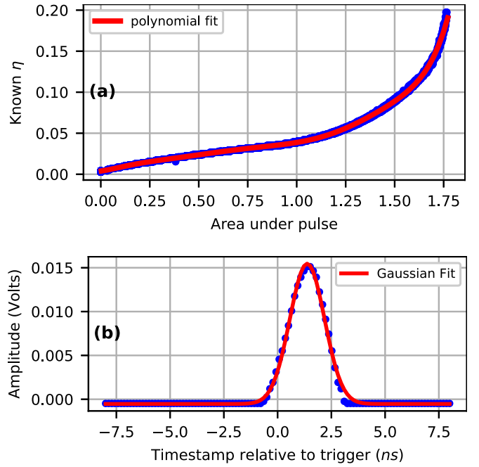
FIG. 6. (a) Polynomial fit to determine the correlation between the measured area under the probe pulse and the programmed transmittance. (b) Example of a probed pulse captured by the oscilloscope and its Gaussian fit.
