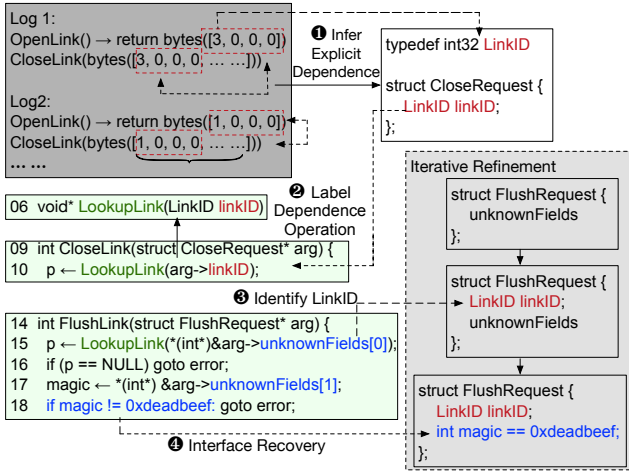
Figure 3: Typical process of interface recovery for the motivating example. ① Inferring explicit dependence by searching for identical input and output pairs from logs; ② Annotating dependence related operations; ③ Identifying more dependence based on annotated code; ④ Recovering structure and constraints of inputs.
