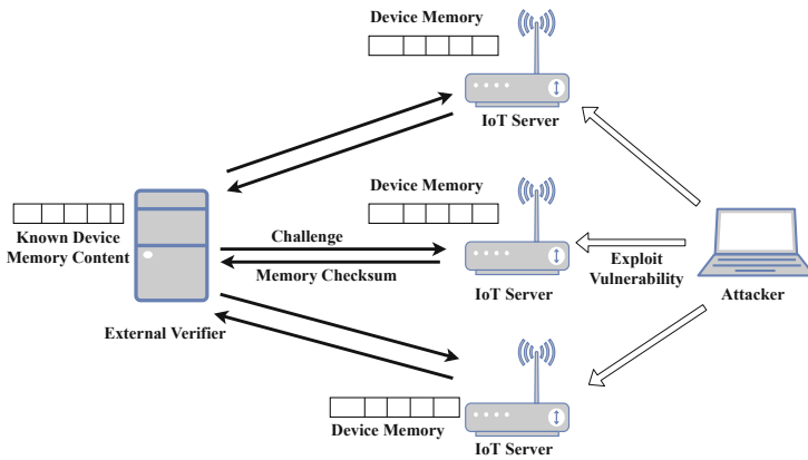
Fig. 1. Remote attestation testbed architecture.
