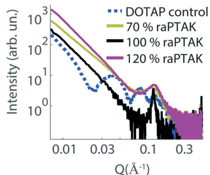
Fig. 6 SAXS intensities of raPTAK/liposome complexes as a function of raPTAK % relative to lipids prepared at room temperature. The dashed blue line shows the pure DOTAP liposome control, whereas solid lines correspond to various raPTAK coverages in raPTAK/liposome complexes.
