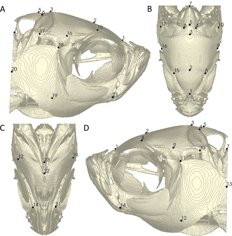
Fig. 4. Gold standard of 23 manual landmarks. Landmark placement represents the average location of two independent landmark placements by the same author. Right lateral (A), dorsal (B), ventral (C), and left lateral (D) views of the atlas mesh are shown. Landmark definitions can be found in Table 3.
