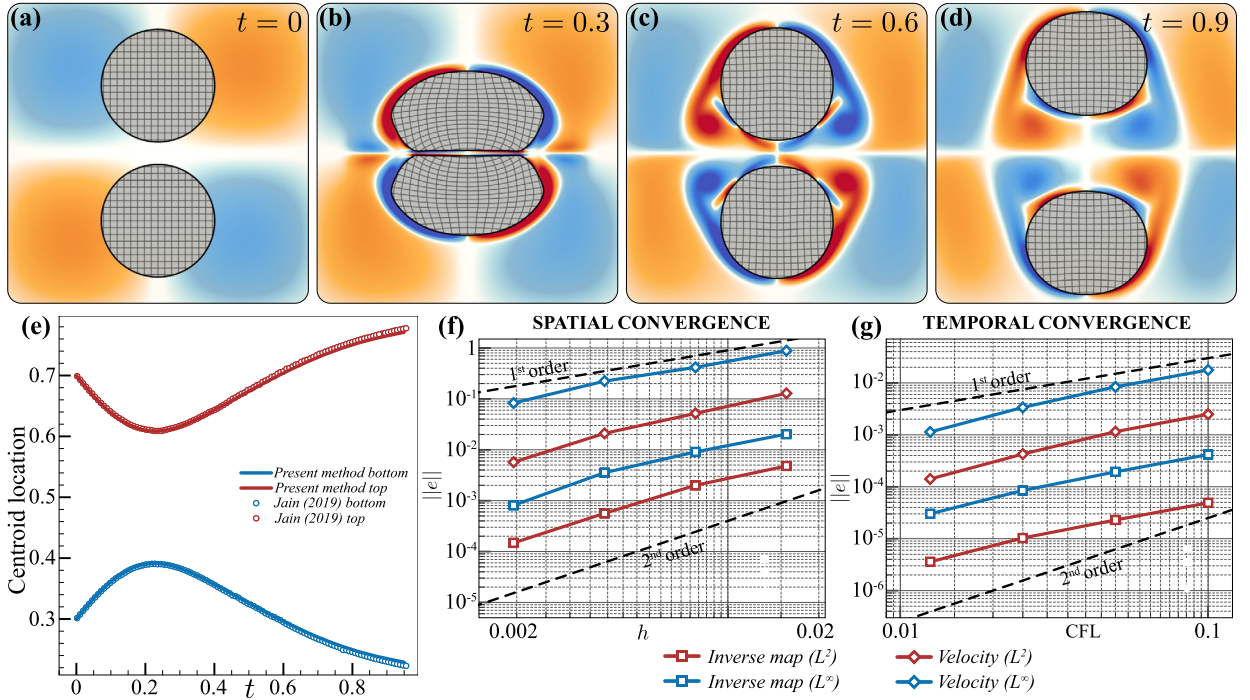
Fig. 5. Collision between two hyperelastic cylinders immersed in a fluid. (a) Case setup. The dynamic parameters corresponding to the fluid phase are \rho_f = 1 , \mu_f = 10^{-2}/2\pi . The neo-Hookean hyperelastic disks, located at (0.5, 0.3) and (0.5, 0.7) , have radii r = 1/6 , are density matched ( \rho_e = \rho_f ), have no internal dissipation ( \mu_e = 0 ), and have shear modulus c_1 = 1.0 i.e. G = 2c_1 = 2.0 . The parameters corresponding to the streamfunction for the imposed vorticity are \psi_0 = 1/2\pi , and L_x = L_y = L = 1 . The key non-dimensional parameters for this benchmark are Re = \rho_f \psi_0 r / \mu_f L = 16.67 and Cau = \rho_e \psi_0^2 / GL^2 = 0.0127 . (b-d) Temporal variation of inverse map (black lines) and vorticity field (orange/blue represent positive/negative vorticity) contours, showing the dynamic response of the cylinders to the initial imposed vorticity. (e) Comparison of temporal variation of the centroids of the cylinders with previous studies [18]. (f) Spatial convergence: L_\infty (blue) and L_2 (red) norms of the error are plotted against grid spacing h , for the inverse map and velocity. (g) Temporal convergence: L_\infty (blue) and L_2 (red) norms of the error are plotted against CFL, for the inverse map and velocity.
