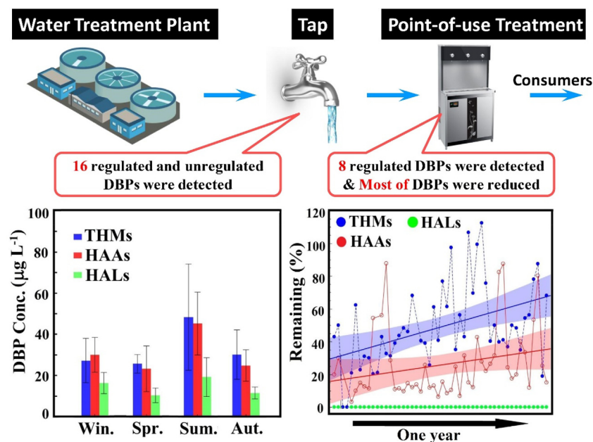
Fig. 2. Typical DBP occurrence at the tap and after treatment by a POU device in a one-year long survey. Reproduced from (Wang et al., 2019) with permission from Elsevier.
