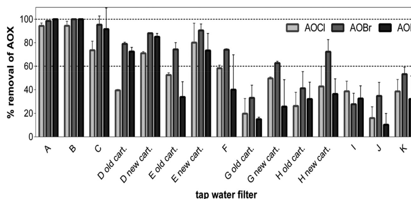
Fig. 4. AOX removal by various water filters (A: RO; B: ceramic outer shell with GAC and activated alumina core; C, E, F: ceramic outer shell with GAC core; G: AC and ion-exchange resin; D, H, J, K: CB; I: activated alumina without carbon). For filters D, E, G, H, results are given before (old cart.) and after filter cartridge replacement (new cart.). Displayed is the arithmetic mean \pm standard deviation ( n = 2-6 ). Reproduced from (Stalter et al., 2016b) with permission from Royal Society of Chemistry.
