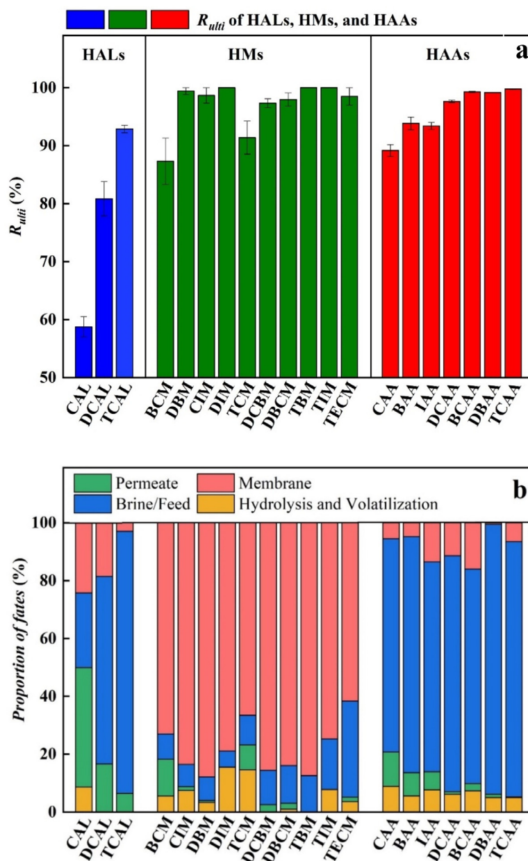
Fig. 6. a) DBP rejection using RO and b) DBP fates during RO operation. Reproduced from (Chen et al., 2021b) with permission from Elsevier.
