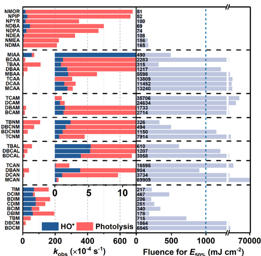
Fig. 7. The observed rate constants of DBPs induced by \bullet\text{OH} and LPUV direct photolysis in UV/ \text{H}_2\text{O}_2 AOP, and the fluence required to degrade half of the DBP concentration ( E_{50\%} ) when I_0 = 5.0 \text{ mW cm}^{-2} , \text{pH} = 7.0 , and [\bullet\text{OH}]_{ss} = 9.83 \times 10^{-13} \text{ M} . The inset enlarges the bars from MIAA to MCAN. Reproduced from (Lei et al., 2020) with permission from Elsevier.
