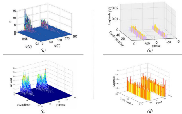
FIGURE 57. Typical PRPD patterns for contaminated insulator from the experimental models reported in: (a) [78], (b) [77], (c) [140], and (d) [141].
