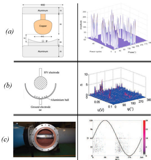
FIGURE 49. Floating particle model and corresponding PRPD: (a) sphere diameter 1mm (10kV HV electrode) and concave ground electrode [134], (b) HV ball electrode with 44mm diameter and half hollow sphere ground electrode 120mm [78], (c) flat metal washer with the diameter of 33mm suspended by insulation tape in real 220kV GIS [135].
