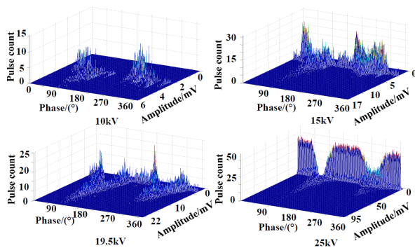
FIGURE 54. Change of the PD pattern with voltage rise for electrode gap defect [136].
