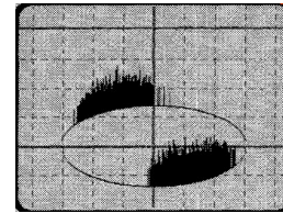
FIGURE 20. Internal discharge PRPD pattern from a large 6.6kV motor in off-line experiment [100].
