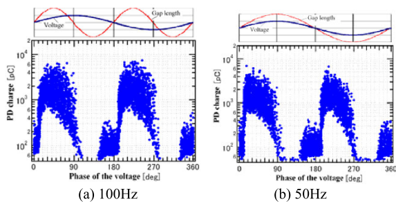
FIGURE 29. PD patterns at two vibration frequencies and lead phase of 180 deg and the applied voltage is 6 kV [15], [113].
