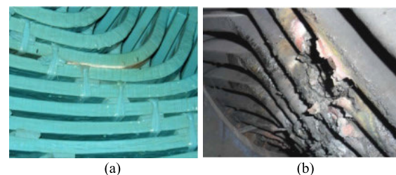
FIGURE 5. (a) Bar-to-bar discharge between stator coils of different phases of the motor ( \geq 6\text{kV} ) [19]; (b) bar-to-bar discharge between stator bars of 10kV motors [18].
