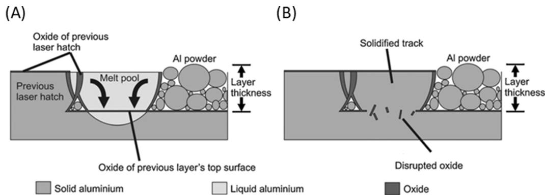
Fig. 33. Schematics of oxide formation in melt pools of aluminum alloy. Reprinted with permission from Ref. [490].
