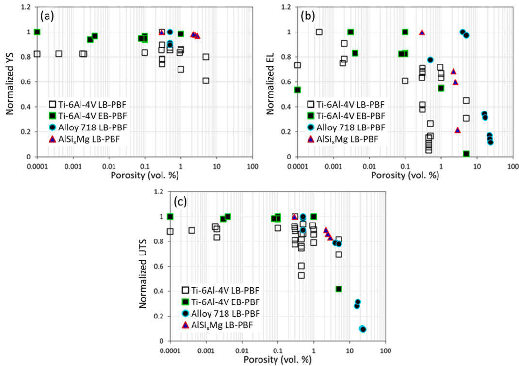
Fig. 97. Plots of normalized (a) YS, (b) Elongation to Failure (EL), and (c) UTS of AM Ti-6Al-4V, Alloy 718, and AlSi x Mg ( x = 10 and 12 ) vs. porosity. Data are collected from Refs. [176,215,984,987,991–996]. The normalization was performed based on the respective maximum values for each material, which are listed in Table 5. Data for both L-PBF and E-PBF processed Ti-6Al-4V are included, while those for only L-PBF Alloy 718 and AlSi x Mg are included. The dependence of tensile properties for AM 17–4 PH SS on porosity is still lacking in the literature to the authors' best knowledge.
