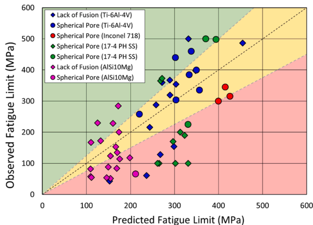
Fig. 103. Observed fatigue limit of various AM alloys vs. the values predicted by the Murakami model. The green region encloses the over-conservative predictions, the brown region encloses the predictions with \pm 25\% accuracy, and the red region encloses under-predictions. Data are obtained from Refs. [215,280,431,432,509,689,762,772,928,944,976,987,1038-1048].
