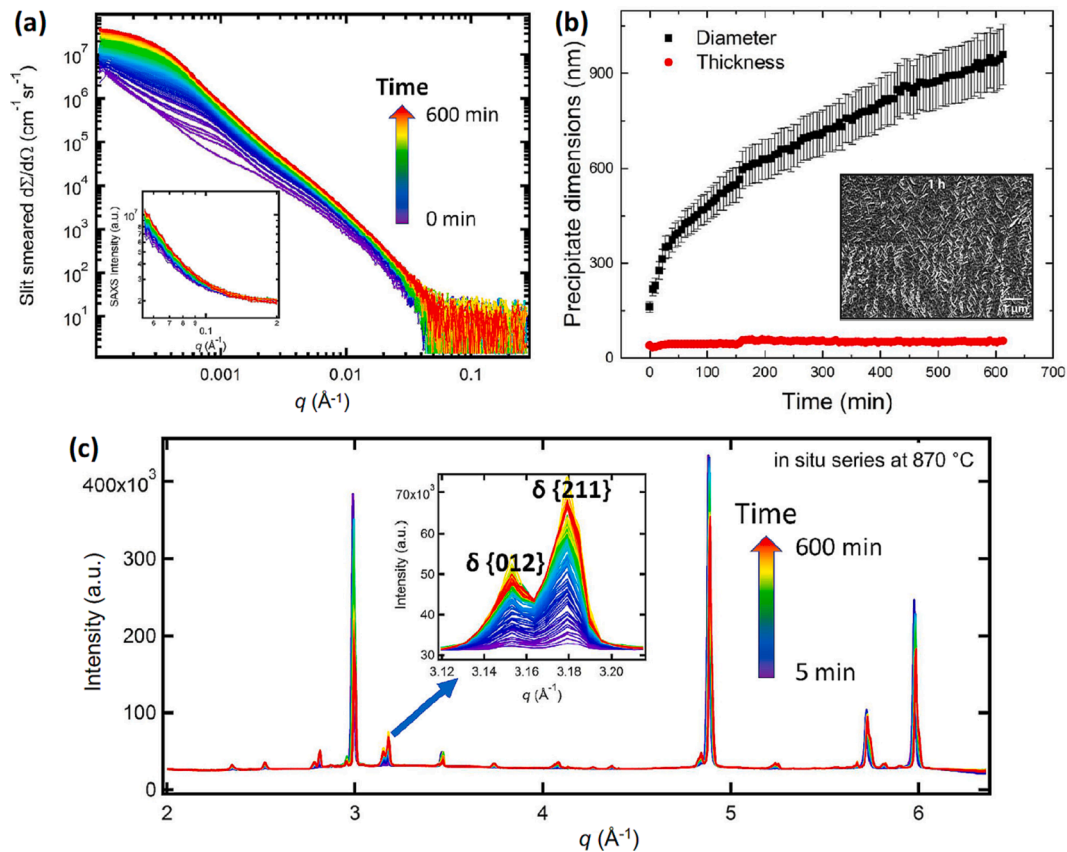
Fig. 14. In situ synchrotron x-ray study of the growth of deleterious \delta phase precipitates in AM alloy 625 during stress-relief heat treatment. (a) A complete set of in situ SAXS data acquired from the alloy 625 sample during isothermal heat treatment at 870 °C for 613 min. The main plot shows the USAXS data, and the inset shows the SAXS data. (b) Time-dependent evolution of average diameter and thickness of the \delta phase. The SEM image of the alloy 625 sample after 1 h is shown in the inset, which reveals the formation of \delta phase precipitates. (c) In situ XRD results during the isothermal heat treatment show the growth of \delta phase. Reprinted with permission from Ref. [250].
