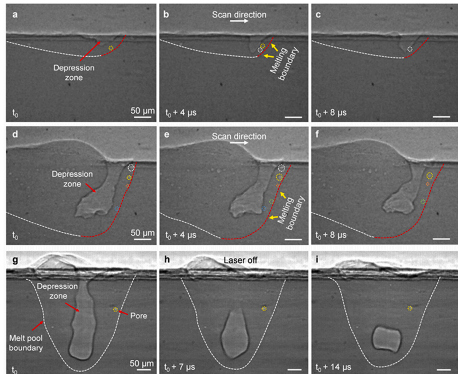
Fig. 71. Pore formation in melt pool boundary during laser melting of aluminum alloys. Pores are displayed by yellow dash circles and melt pool boundaries are shown by red dotted lines. Reprinted with permission from Ref. [537].
