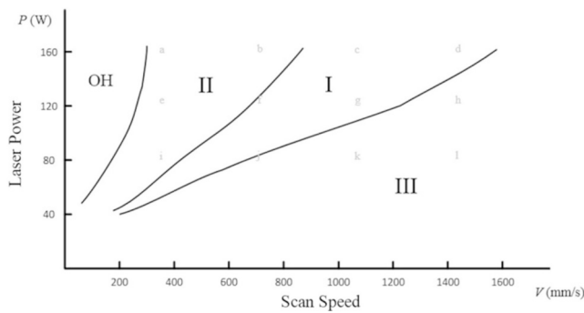
Fig. 73. Processing map. Zone I - fully dense; zone II - subsurface porosity; zone III - insufficient melting; OH - serious surface deformation. Reprinted with permission from Ref. [84].
