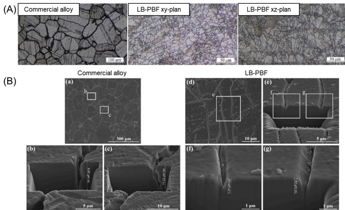
Fig. 105. (A) Optical micrographs after DL-EPR tests (0.5 M H_2SO_4 + 0.01 M KSCN solution at room temperature). (B) Focused ion beam cross-sections from the grain boundaries of specimens to measure the depth of attack. Reprinted with permission from Ref. [1093].
