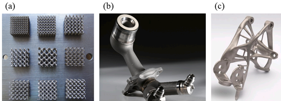
Fig. 2. Examples of AM geometries. (a) Complex lattice structures. Reprinted with permission from Ref. [20]. (b) Fuel nozzle printed by GE. Reprinted with permission from Ref. [21]. (c) Lightweight seat bracket produced by GM. Reprinted with permission from Ref. [22].
