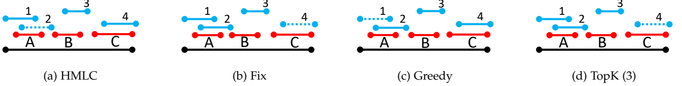
Fig. 4: Illustration of alternative assignment strategies. The notations are the same as Fig. 3. Different assignment strategies will assign the predicted segments to the ground truth segments differently; solid blue lines indicate matched predictions, dashed blue lines indicate unmatched predictions. (a) HMLC matching (1-A, 3-B, 4-C); (b) Fixed order matching (1-A, 2-B, 3-C); (c) Greedy matching (2-A, 3-B, 4-C); (d) TopK matching for K = 3 (2-A, 3-B, 1-C)
