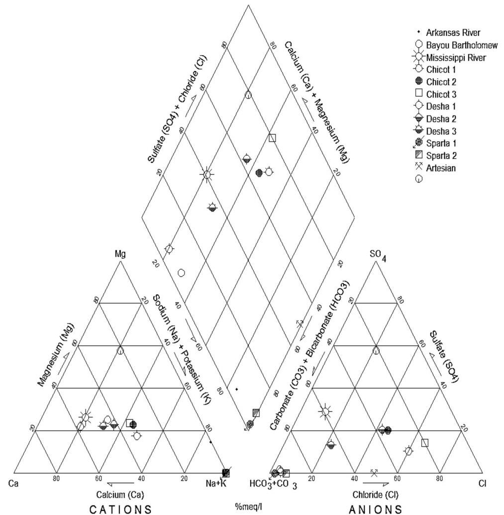
Fig. 5 Piper diagram showing composition of groundwater samples collected in this study and streams in the study area, including the Arkansas River, Bayou Bartholomew, and Mississippi River (from Paul 2015). Stream data from USGS (USGS NWIS 2014)
